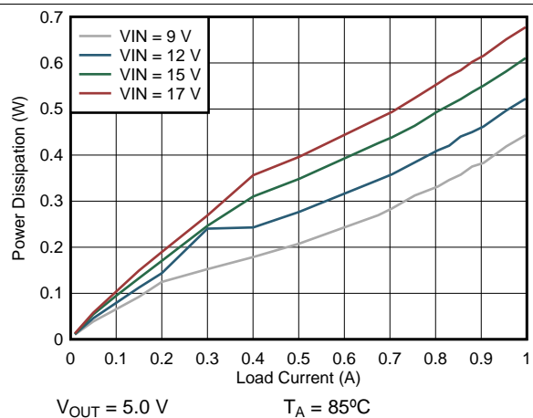
Figure 5. Power Dissipation
