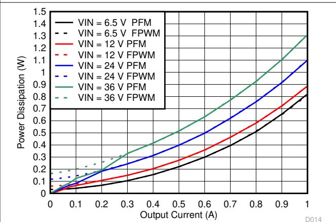
6-10. Power Dissipation
