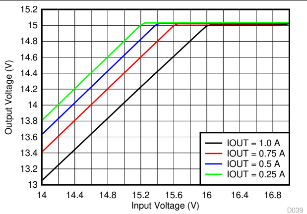
6-4. Dropout Voltage
