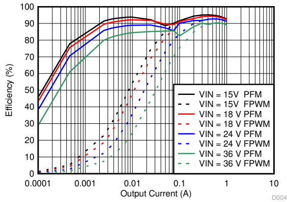
8-18. Efficiency
