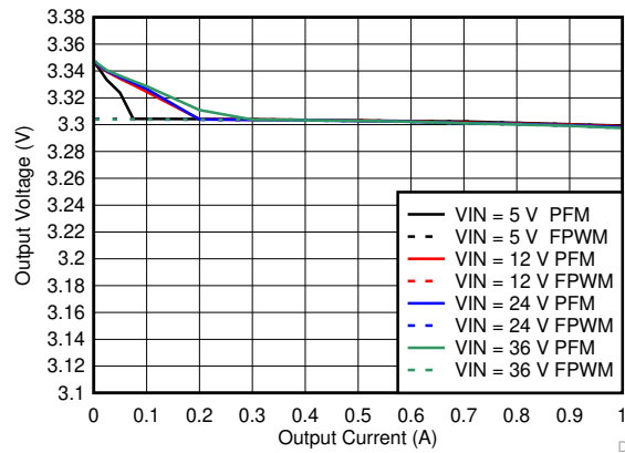
8-45. Line and Load Regulation for V_{OUT} = 3.3\text{ V}
