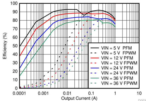
8-12. Efficiency
