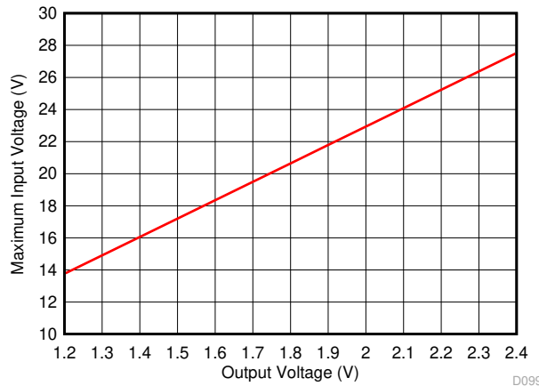
6-1. Maximum Input Voltage for V_{OUT} < 2.5\text{V}
