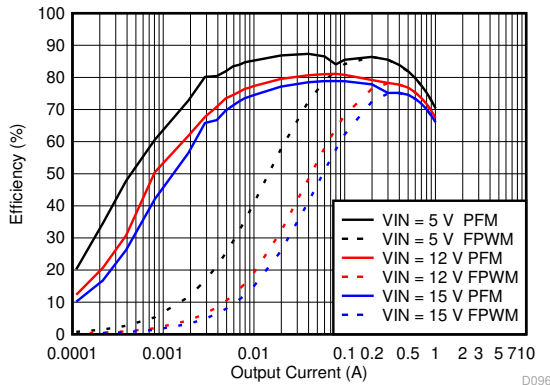
8-36. Efficiency for V_{OUT} = 1.8\text{ V}
