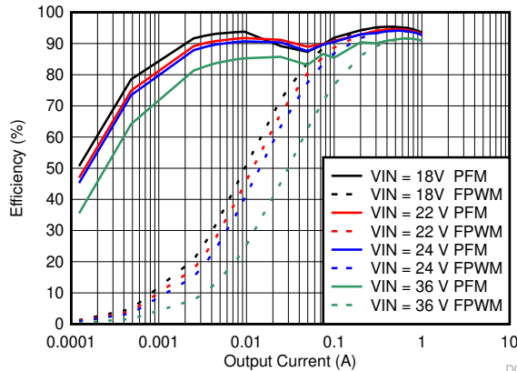
8-24. Efficiency
