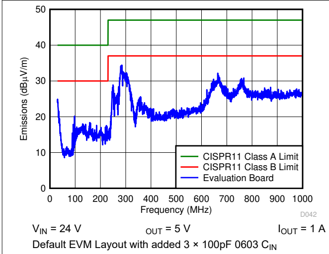
6-7. Radiated EMI
