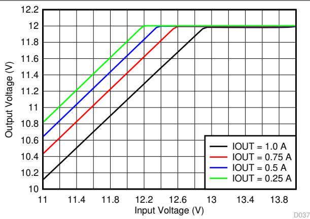
6-3. Dropout Voltage
