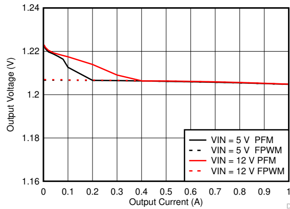
8-39. Line and Load Regulation for V_{OUT} = 1.2\text{ V}
