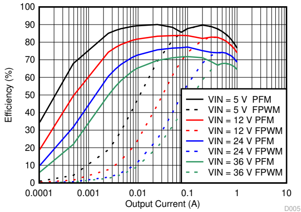
8-30. Efficiency
