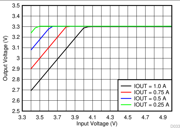
6-3. Dropout Voltage
