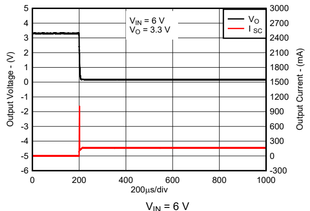
FIG 5-18. Short-Circuit Current vs Time (New Chip)
