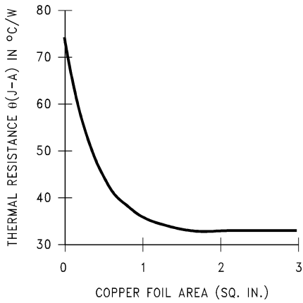
FIGURE 5. \theta_{JA} vs Copper (1 Ounce) Area for TO-263 package
