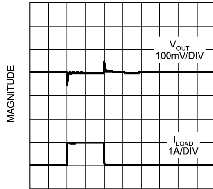
Load Transient Response C_{IN} = C_{OUT} = 100\mu\text{F} , TANTALUM
