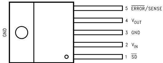
Top View TO220-5 Package Bent, Staggered Leads
