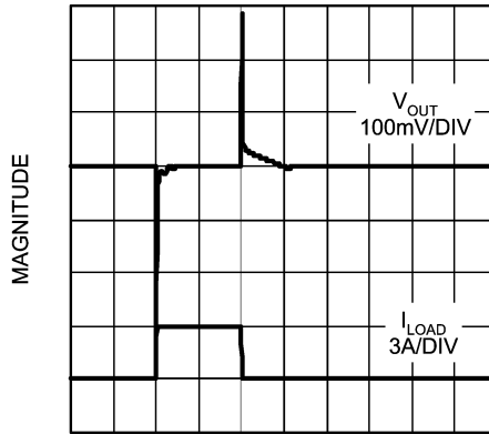
Load Transient Response C_{IN} = C_{OUT} = 10\mu\text{F} , TANTALUM
