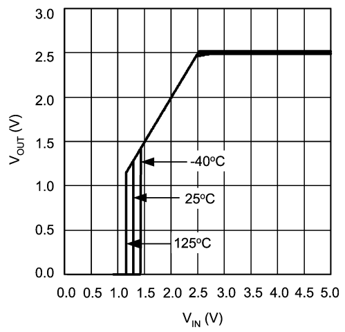
V_{IN} vs V_{OUT} Over Temperature
