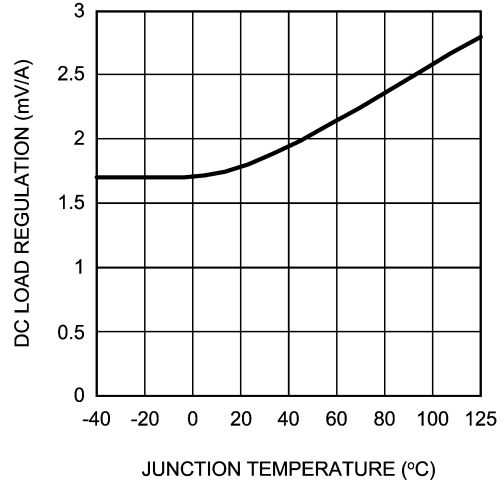
DC Load Reg. vs Junction Temperature
