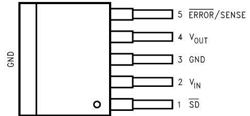
Top View TO263-5 Package
