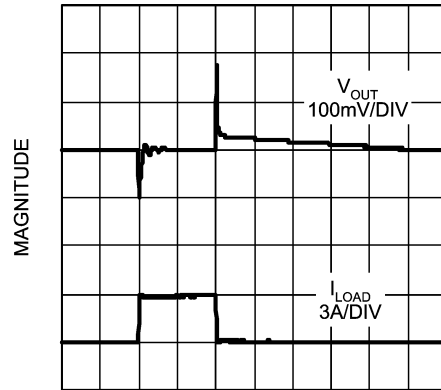
Load Transient Response C_{IN} = C_{OUT} = 100\mu\text{F} , OSCON
