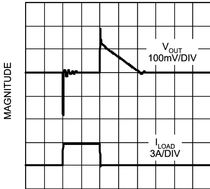
Load Transient Response C_{IN} = C_{OUT} = 10\mu\text{F} , OSCON
