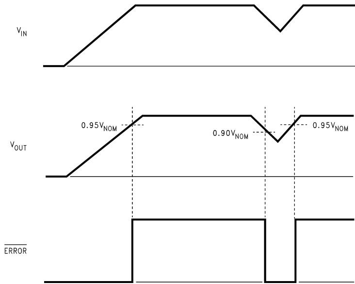
FIGURE 1. Error Flag Operation
