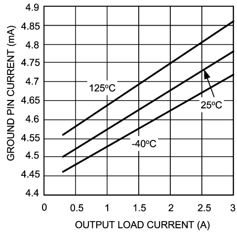
Ground Current vs Output Load Current V_{OUT} = 5\text{A}
