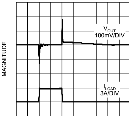
Load Transient Response C_{IN} = C_{OUT} = 100\mu\text{F} , POSCAP
