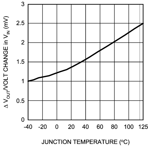
DC Line Regulation vs Temperature
