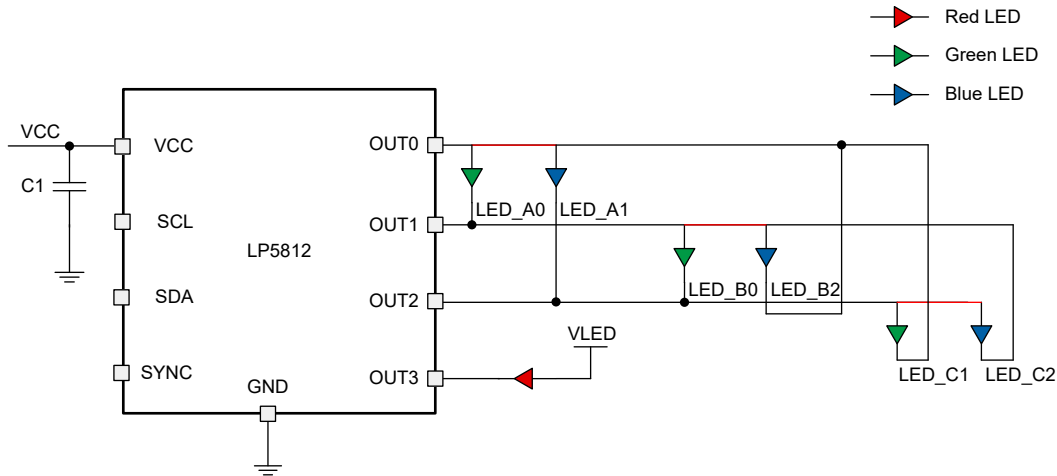
図 8-10. 混在駆動モード、3 スキャン ( led\_mode = 7h , scan\_order\_0 = 0h , scan\_order\_1 = 1h , scan\_order\_2 = 2h , mix\_sel\_led = 8h )
