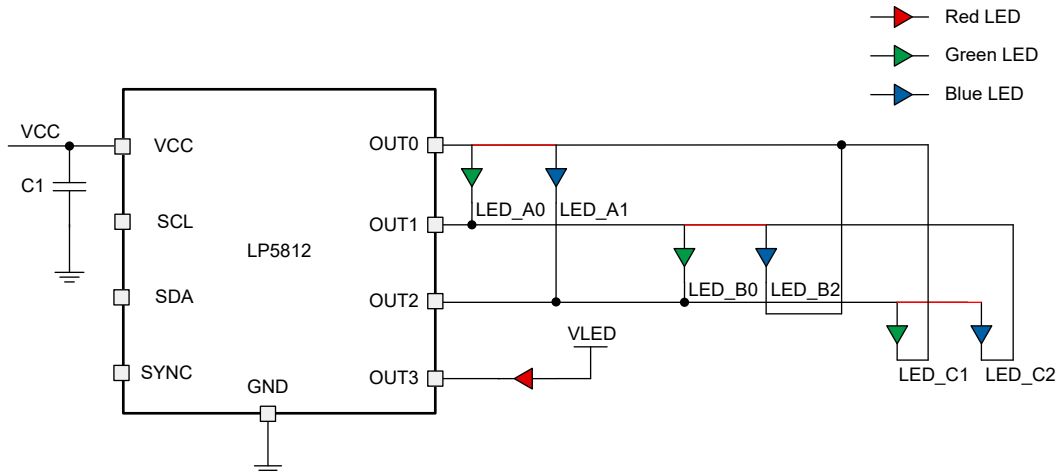
図 6-10. 混在駆動モード、3 スキャン ( led\_mode = 7h , scan\_order\_0 = 0h , scan\_order\_1 = 1h , scan\_order\_2 = 2h , mix\_sel\_led = 8h )
