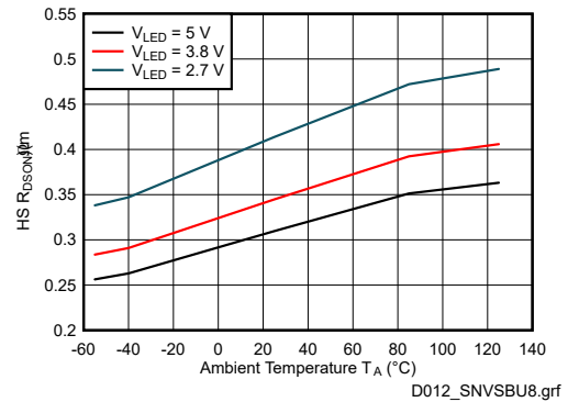
7-10. High Side Switch R_{DS(on)}
