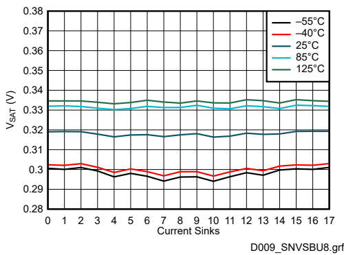
7-7. V_{SAT} vs Current Sinks (30 mA)
