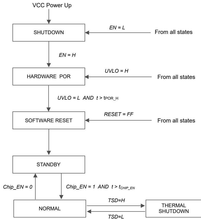
8-10. Device Functional Modes
