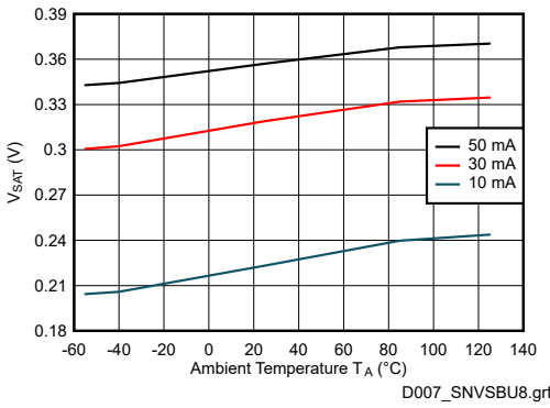
7-5. V_{SAT} vs Temperature
