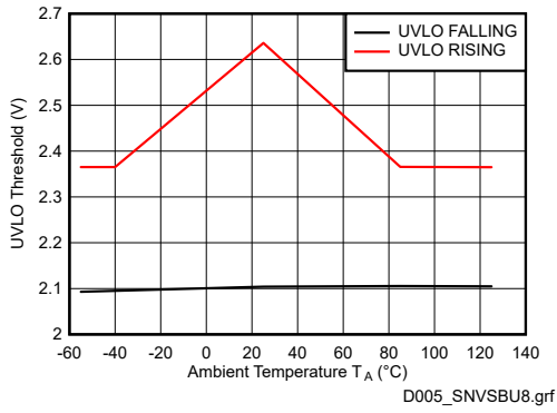
7-3. V_{CC} UVLO Rising and Falling Thresholds
