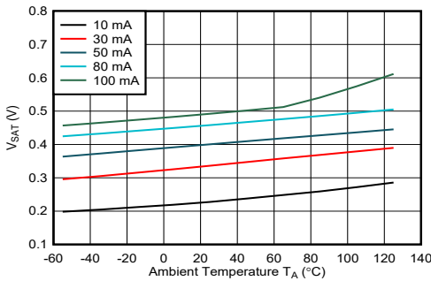
6-5. V_{SAT} vs Temperature
