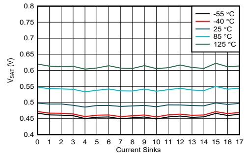
6-6. V_{SAT} vs Current Sinks (100mA)
