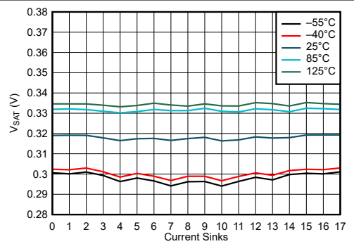
6-8. V_{SAT} vs Current Sinks (30mA)
