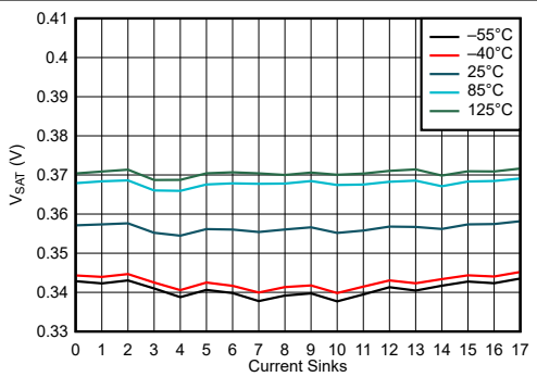
6-7. V_{SAT} vs Current Sinks (50mA)
