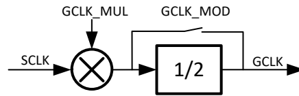
图 7-6. Frequency Multiplier Block Diagram
