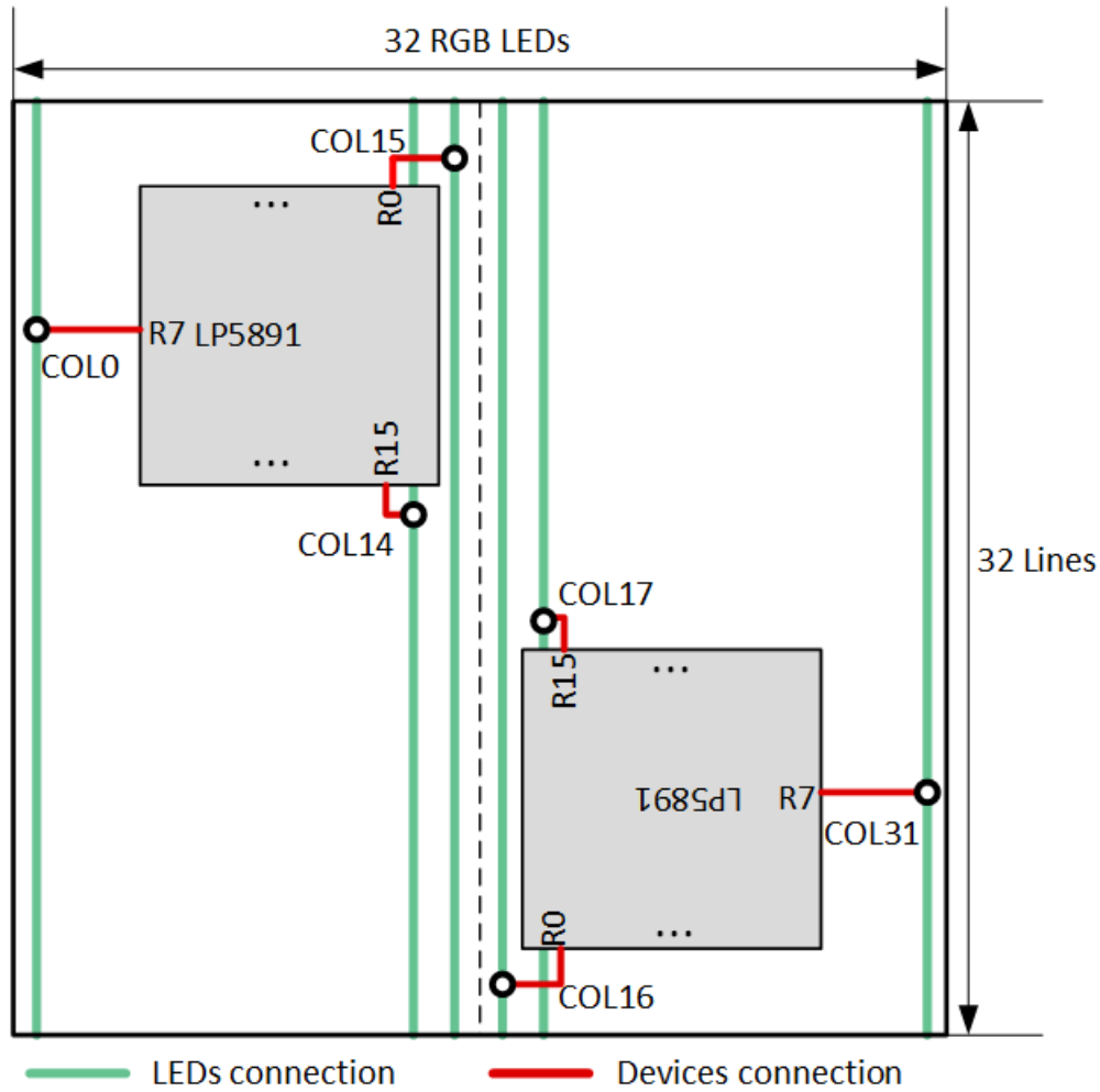
☒ 10-3. Channel Routing Suggestion with Shortest Wire
