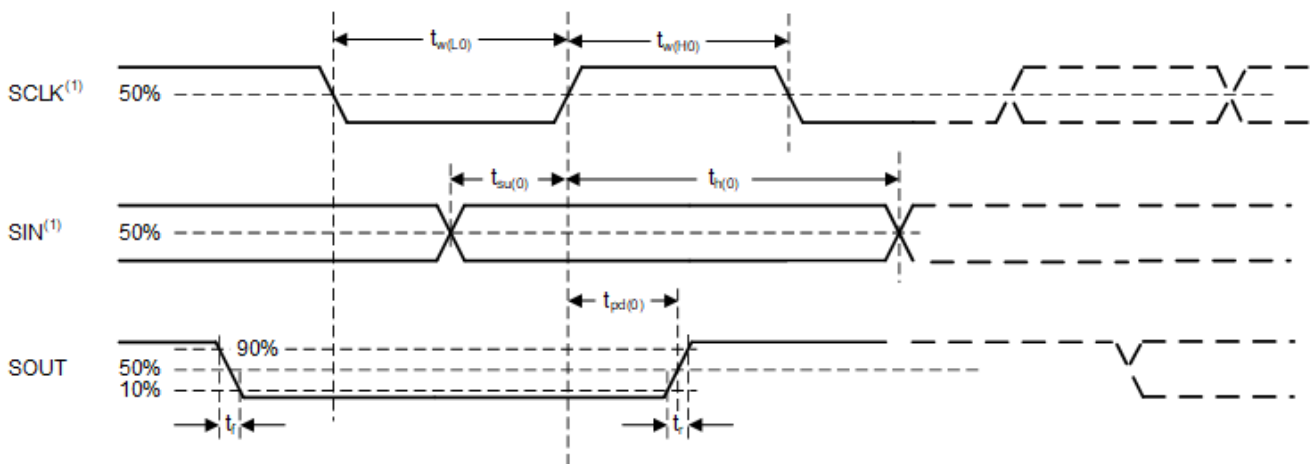
6-1. Timing and Switching Diagram
