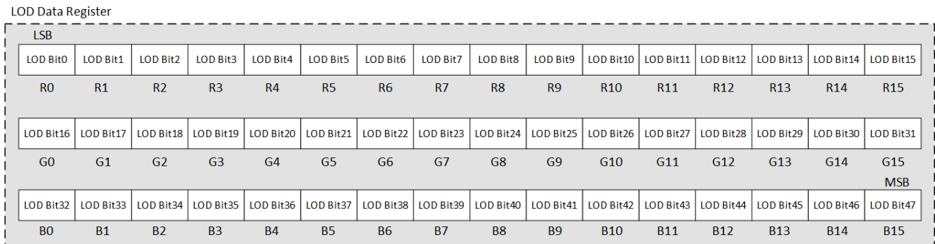
7-9. Bit Arrangement in LOD Data Register
