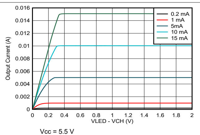
6-3. Channel Current vs (VLED-Vchannel) Voltage
