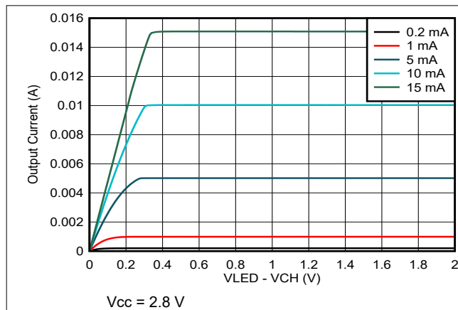
6-2. Channel Current vs (VLED-Vchannel) Voltage
