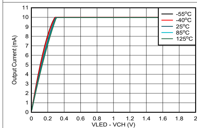
6-4. Channel Current vs (VLED-Vchannel) Voltage
