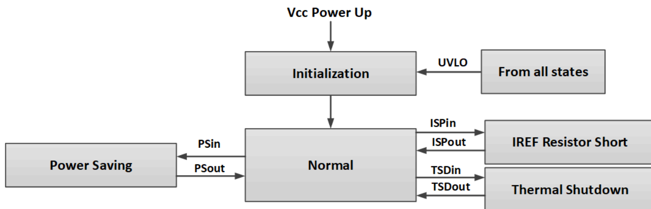
Figure 7-16. Functional Modes
