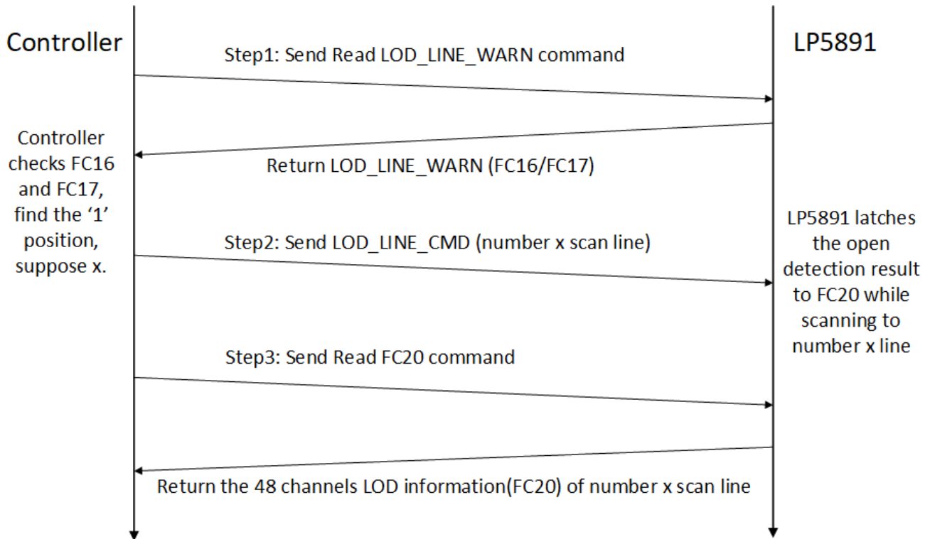
7-10. Steps to Read LED Open Information
