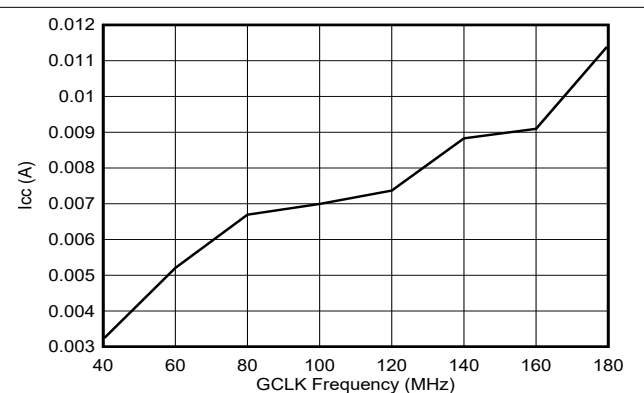
6-7. I CC Current vs GCLK Frequency
