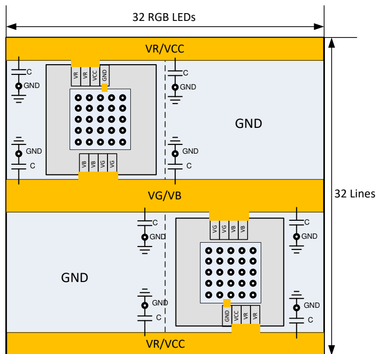
10-1. Power Rails Routing Suggestion
