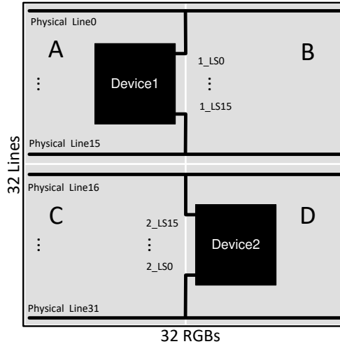
7-2. Mode2 Diagram
