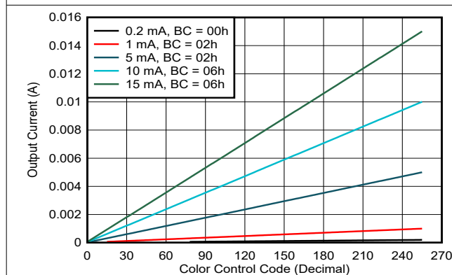
6-6. Color Control Code vs Output Current
