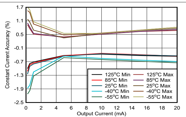
6-5. Channel to Channel Accuracy vs Output Current
