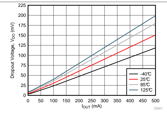
Figure 44. LP5912-1.8 Dropout Voltage ( V_{DO} ) vs I_{OUT}
