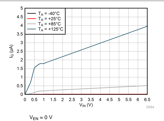
Figure 14. LP5912-0.9 I_{Q(SD)} vs V_{IN}
