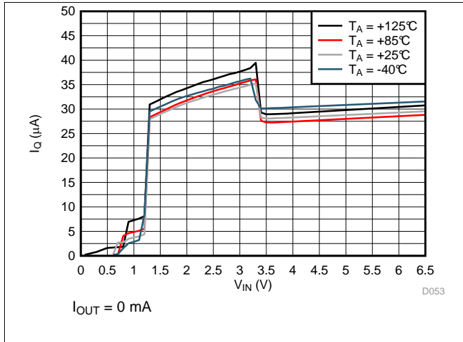
Figure 13. LP5912-3.3 I_Q (No Load) vs V_{IN}
