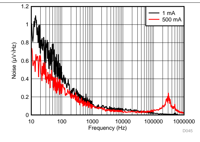
Figure 48. LP5912-3.3 Noise vs Frequency
