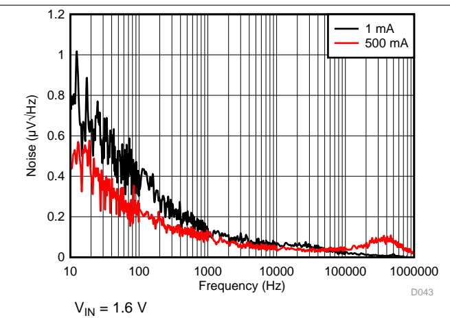
Figure 46. LP5912-0.9 Noise vs Frequency
