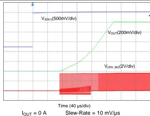
图 67. Start-Up With EN1, Forced PWM (2-Phase Output)
