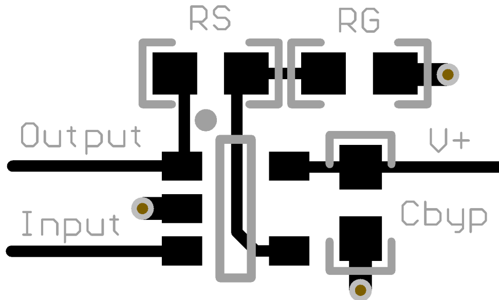
☒ 7-9. Noninverting Layout Example
