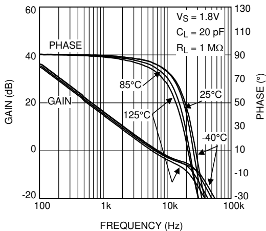
5-41. Frequency Response vs Temperature
