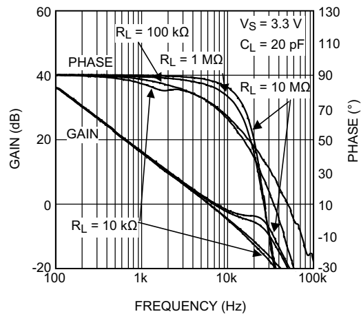
図 5-45. Frequency Response vs R_L
