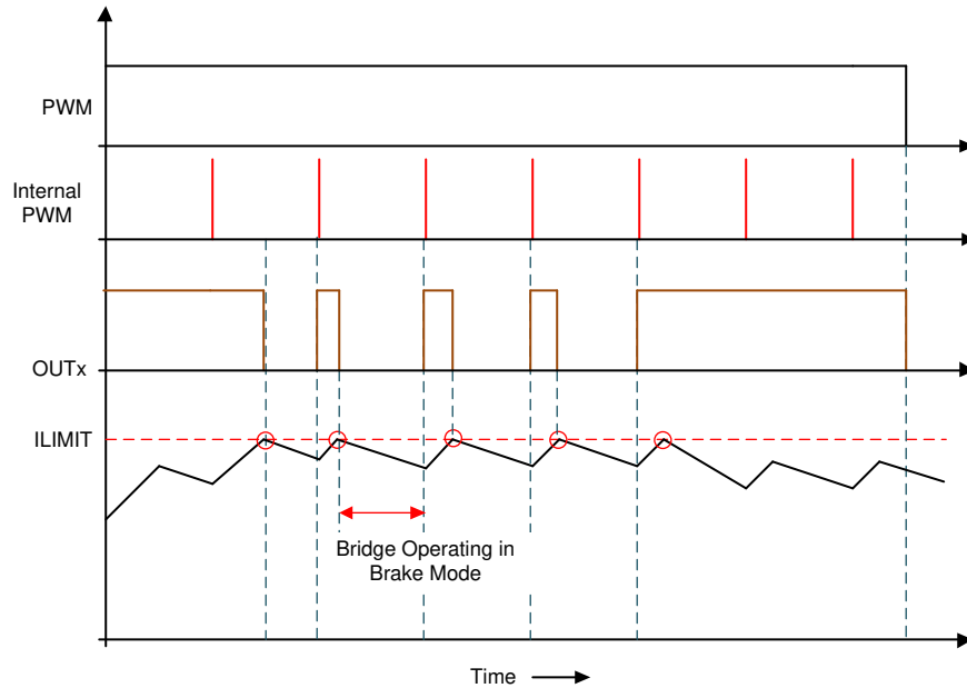
图 7-26. Cycle-by-Cycle Current-Limit Operation with 100% PWM Duty Cycle
