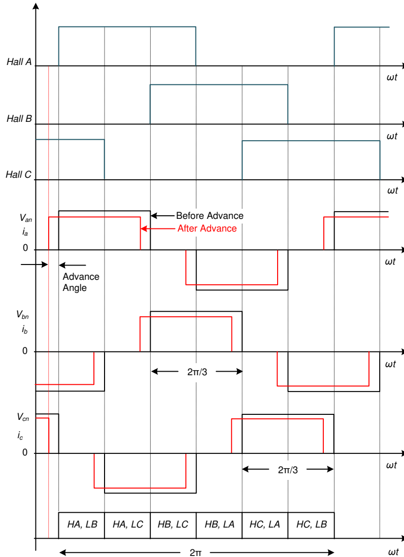
☒ 7-28. Advance Angle
