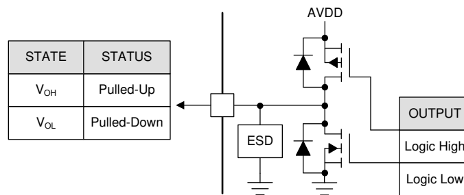
7-17. Push Pull
