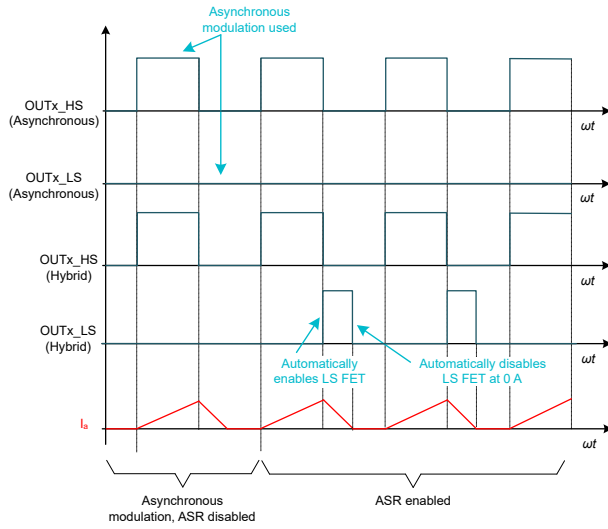
Figure 7-19. Comparing Asynchronous Modulation and ASR
