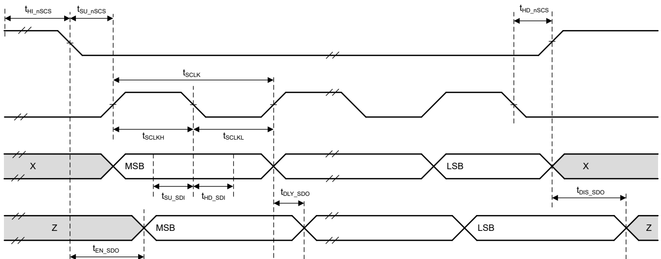
図 6-1. SPI Secondary Device Mode Timing Diagram
