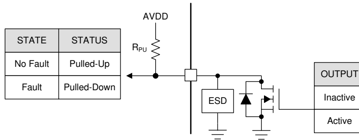
7-16. Open Drain
