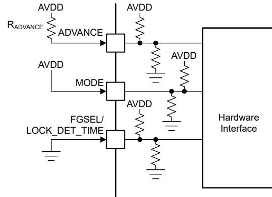
7-8. MCT8314ZZH Hardware Interface
