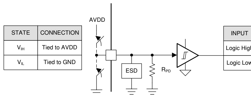
7-14. Logic-Level Input Pin Structure
