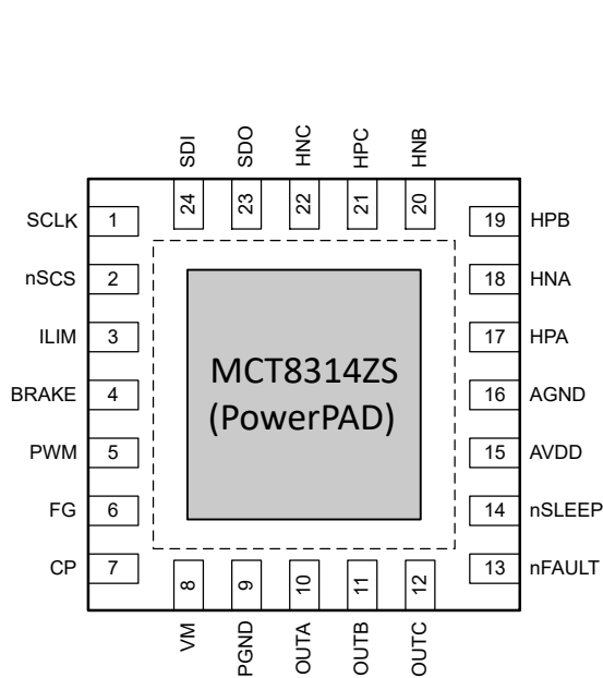
図 5-1. MCT8314ZS 24-Pin VQFN With Exposed Thermal Pad Top View
