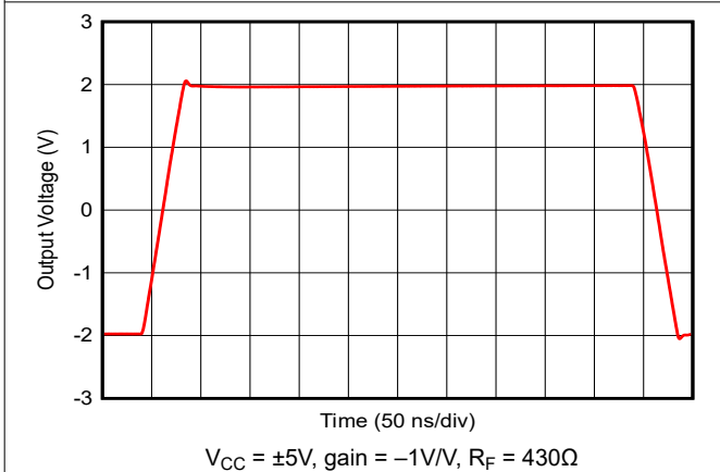
5-23. 4V Step Response
