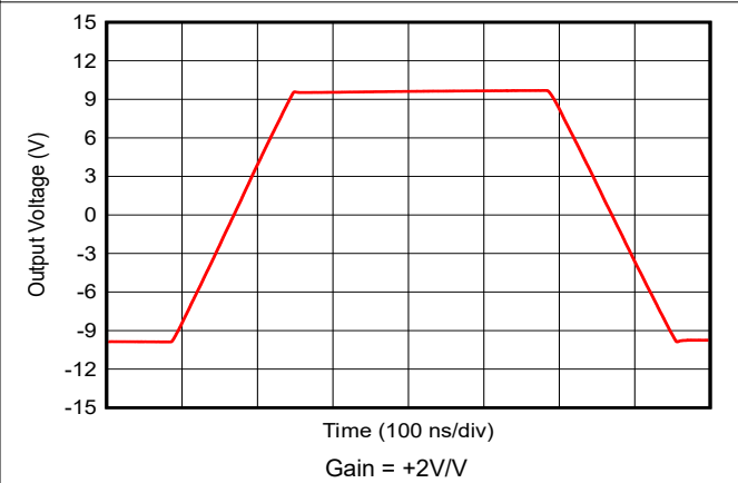
5-24. 20V Step Response
