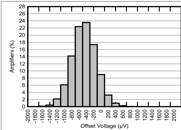
Distribution from 17,184 amplifiers
