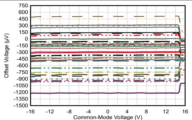
Each line represents one channel T_A = 125^\circ\text{C}
