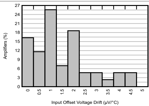
Distribution from 43 amplifiers T_A = -40^\circ\text{C} to 125^\circ\text{C}
