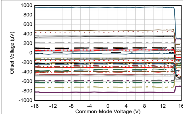
Each line represents one channel T_A = 25^\circ\text{C}
