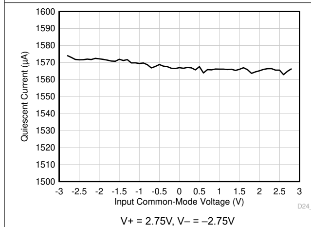
Figure 6-51. Quiescent Current vs Common-Mode Voltage
