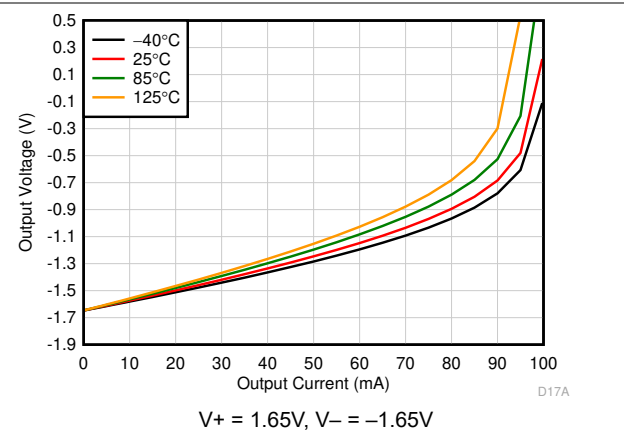
6-26. Output Voltage Swing vs Output Current (Sinking)
