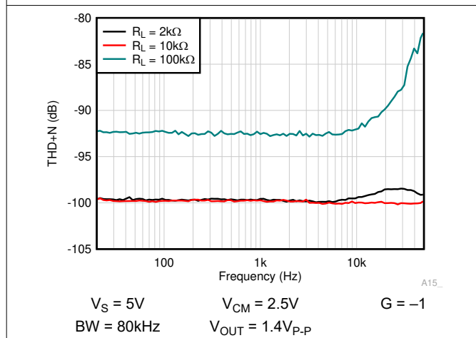
图 6-45. THD + N vs Frequency
