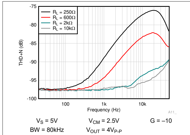
图 6-43. THD + N vs Frequency
