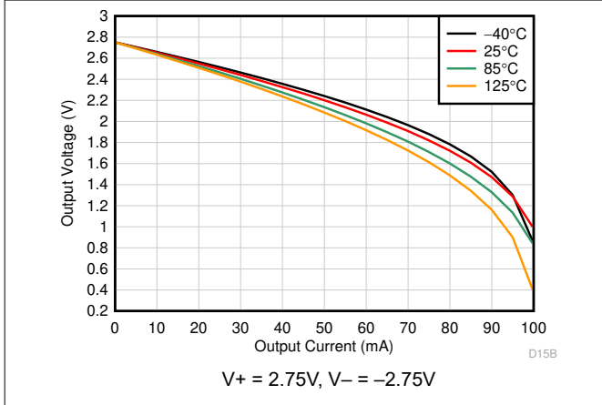
6-23. Output Voltage Swing vs Output Current (Sourcing)
