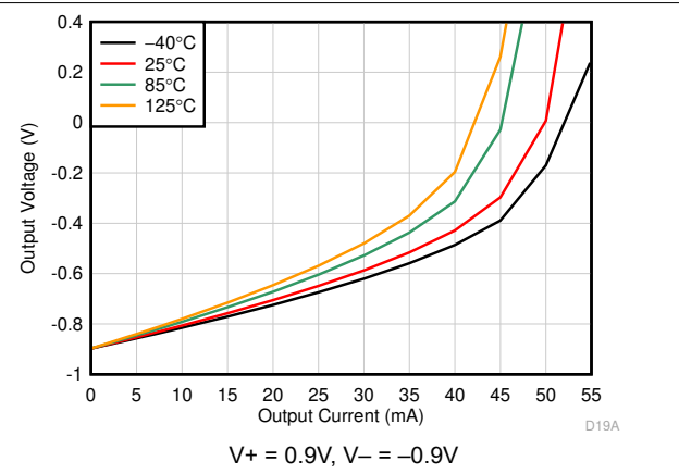
6-28. Output Voltage Swing vs Output Current (Sinking)
