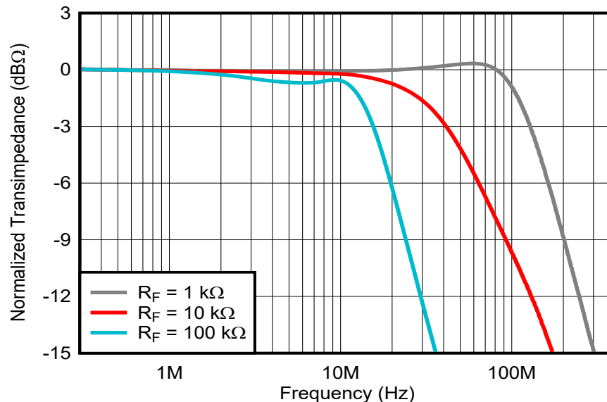
☒ 9-2. Bandwidth vs Frequency
