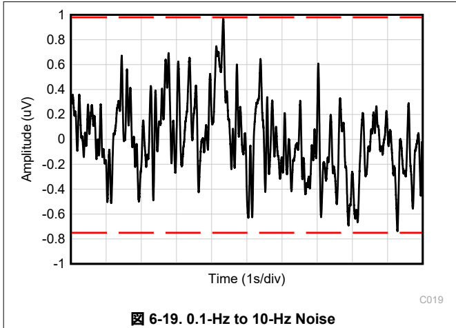
6-19. 0.1-Hz to 10-Hz Noise
