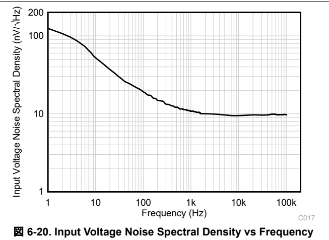
6-20. Input Voltage Noise Spectral Density vs Frequency
