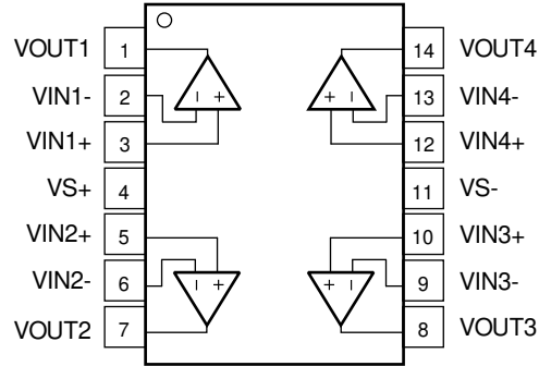
图 6-5. OPA4863 PW Package, 14-Pin TSSOP (Top View)
