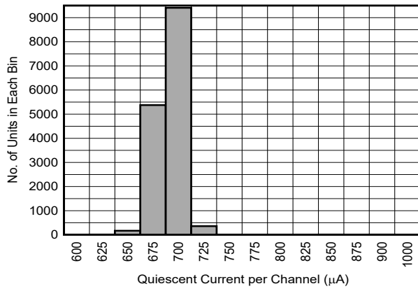
Fig 7-19. Quiescent Current Distribution
