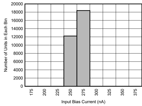
Fig 7-20. Input Bias Current Distribution
