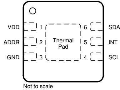
☒ 4-2. DNP Package, 6-Pin USON (Top View)
