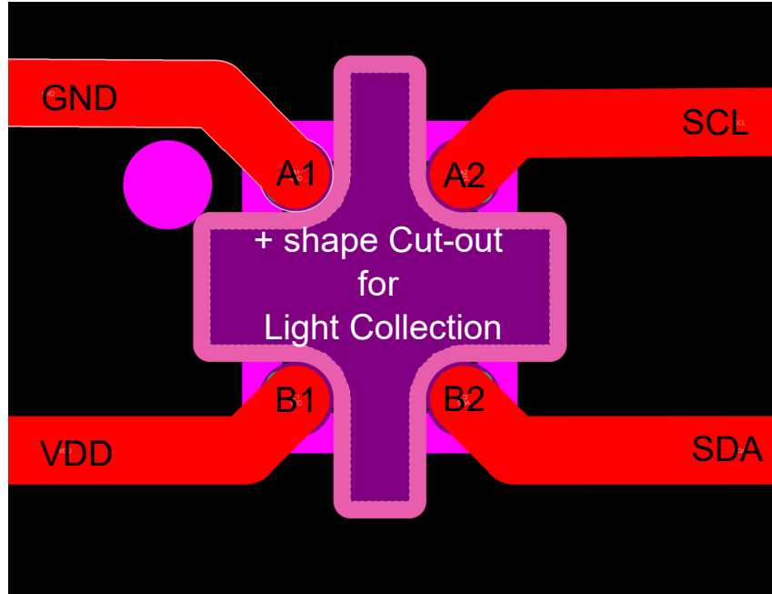
図 8-15. Layout Example for YMN Package With Plus-Shaped Cut Out
