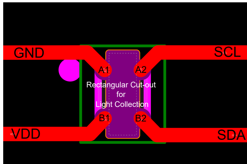
図 8-16. Layout Example for YMN Package With Rectangular Cut Out
