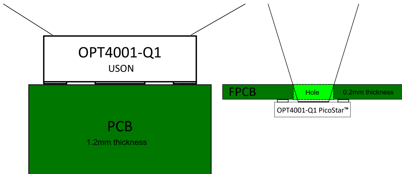
☒ 8-9. Placement Side View of Packages
