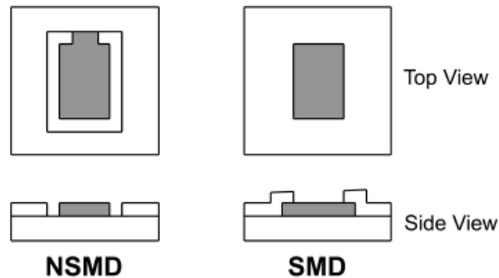
図 8-10. Solder Mask Defined Pad (SMD) and Non-Solder Mask Defined Pad (NSMD)
