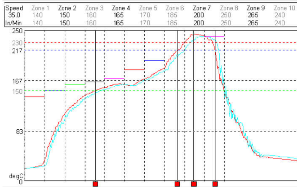
☒ 8-11. Recommended Solder Reflow Temperature Profile
