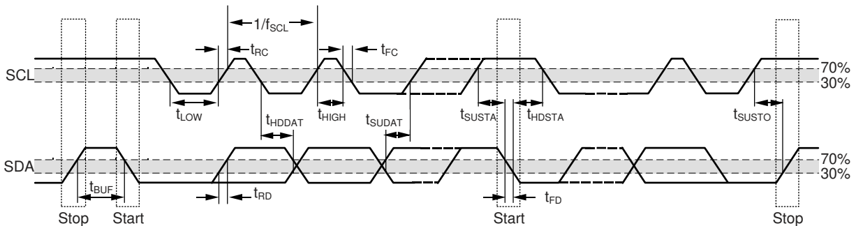
图 5-1. I 2 C Detailed Timing Diagram
