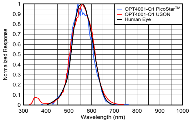
图 5-2. Spectral Response vs Wavelength
