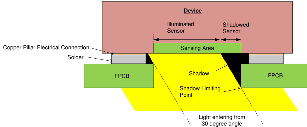
図 8-6. Cross-Sectional Diagram of OPT4001-Q1 Soldered to an FPCB With a Cutout, Including Light Entering From an Angle
