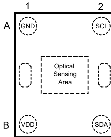
図 4-1. YMN Package, 4-Pin PicoStar™ (Top View)
