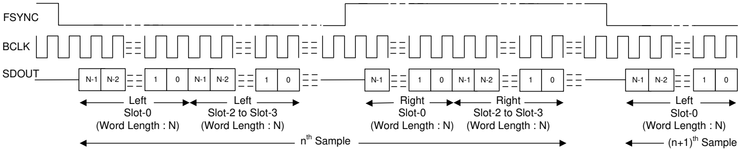
图 7-5. I 2 S Mode Standard Protocol Timing (TX_OFFSET = 0)
