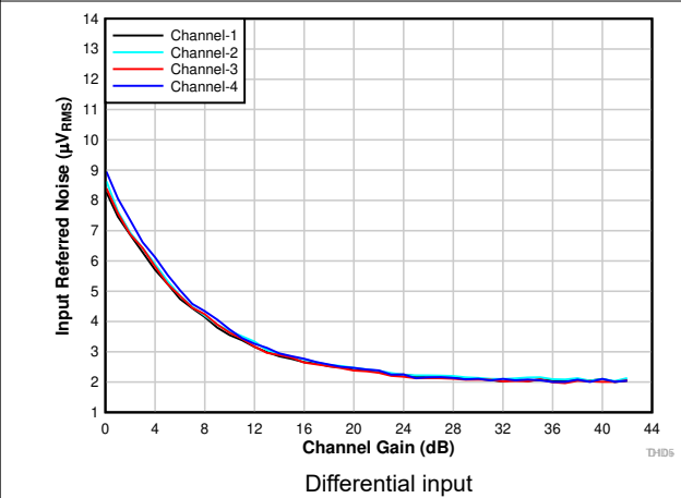
6-13. Input-Referred Noise vs Channel Gain
