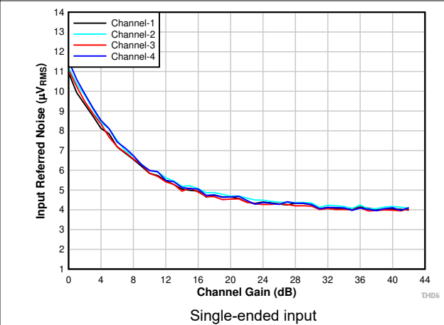
6-14. Input-Referred Noise vs Channel Gain
