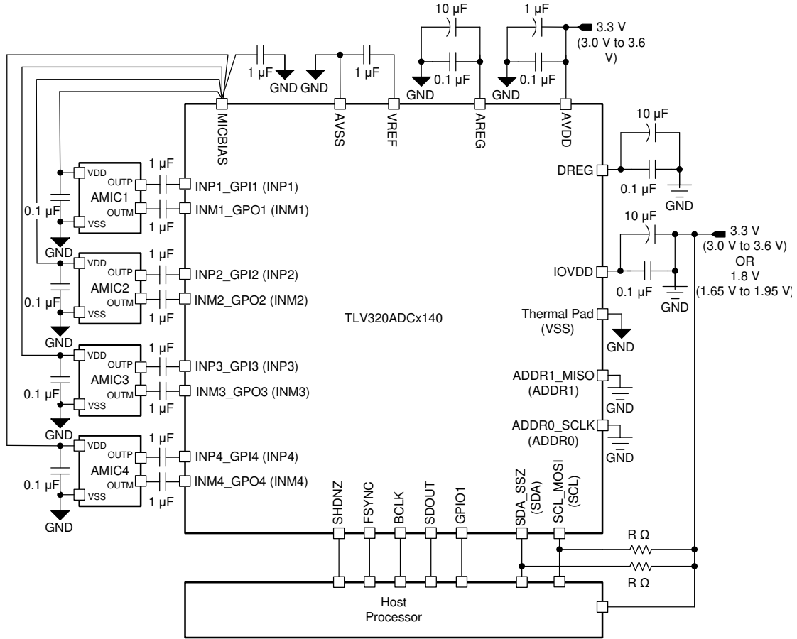
図 8-1. Four-Channel Analog Microphone Recording Diagram
