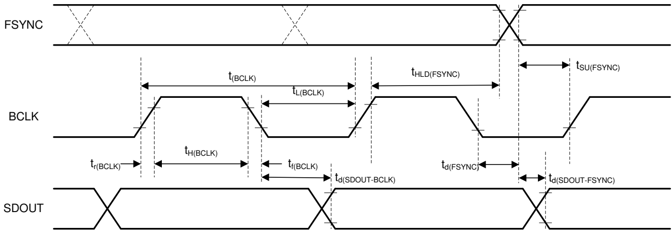
图 6-3. TDM (With BCLK_POL = 1), I 2 S, and LJ Interface Timing Diagram
