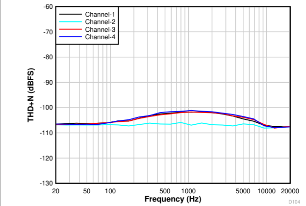
6-12. THD+N vs Input Frequency With a -1-dBr Input
