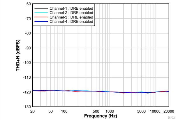
6-11. THD+N vs Input Frequency With a -60-dBr Input
