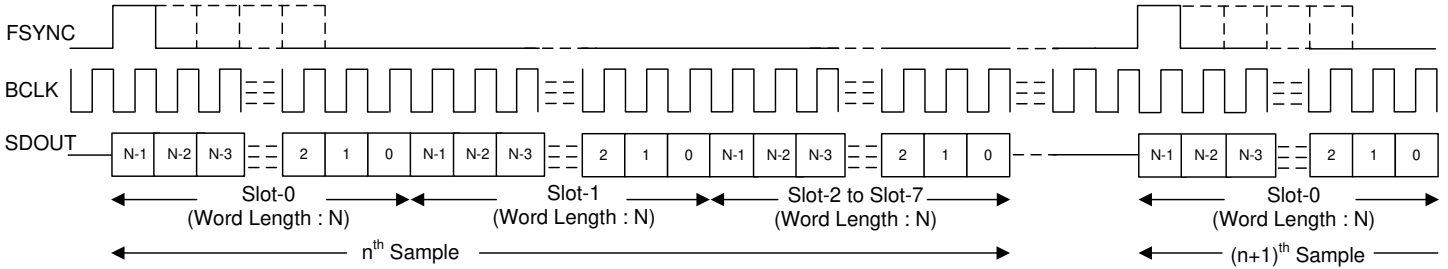
图 7-4. TDM Mode Protocol Timing (TX_OFFSET = 0 and BCLK_POL = 1)
