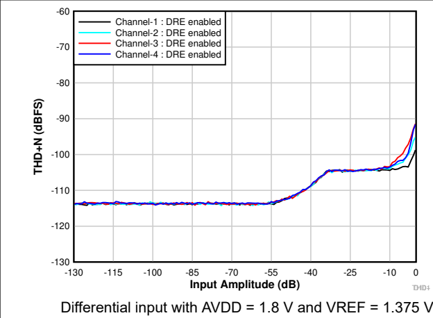
6-9. THD+N vs Input Amplitude With DRE Enabled
