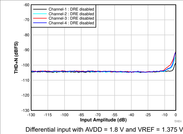
6-10. THD+N vs Input Amplitude With DRE Disabled
