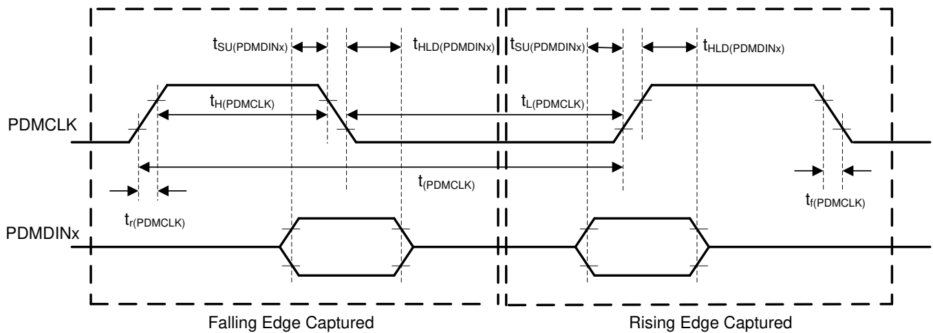
图 6-4. PDM Digital Microphone Interface Timing Diagram
