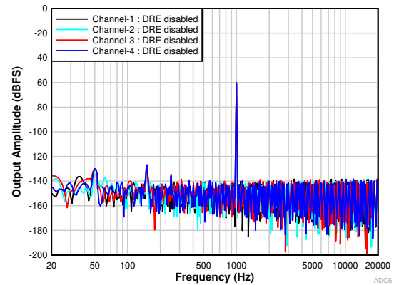
6-20. FFT With a -60-dBr Input With DRE Disabled
