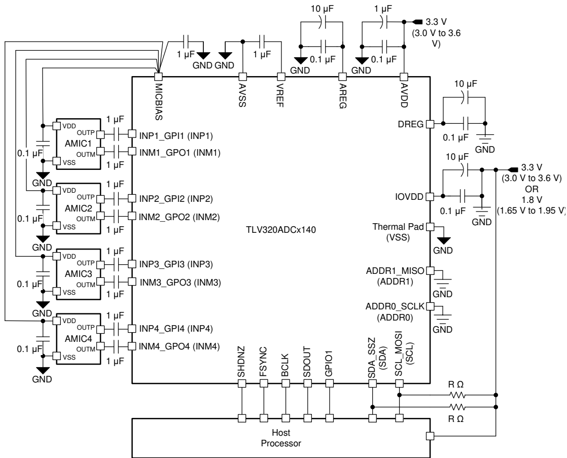
図 8-1. Four-Channel Analog Microphone Recording Diagram
