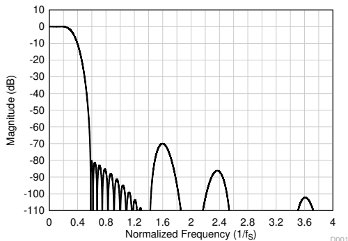
☒ 7-33. Linear Phase Decimation Filter Magnitude Response
