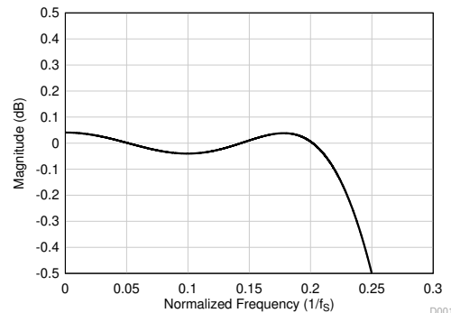
☒ 7-34. Linear Phase Decimation Filter Pass-Band Ripple
