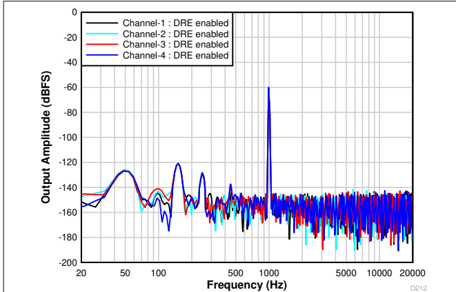
8-2. FFT With a -60-dBr Input With DRE Enabled
