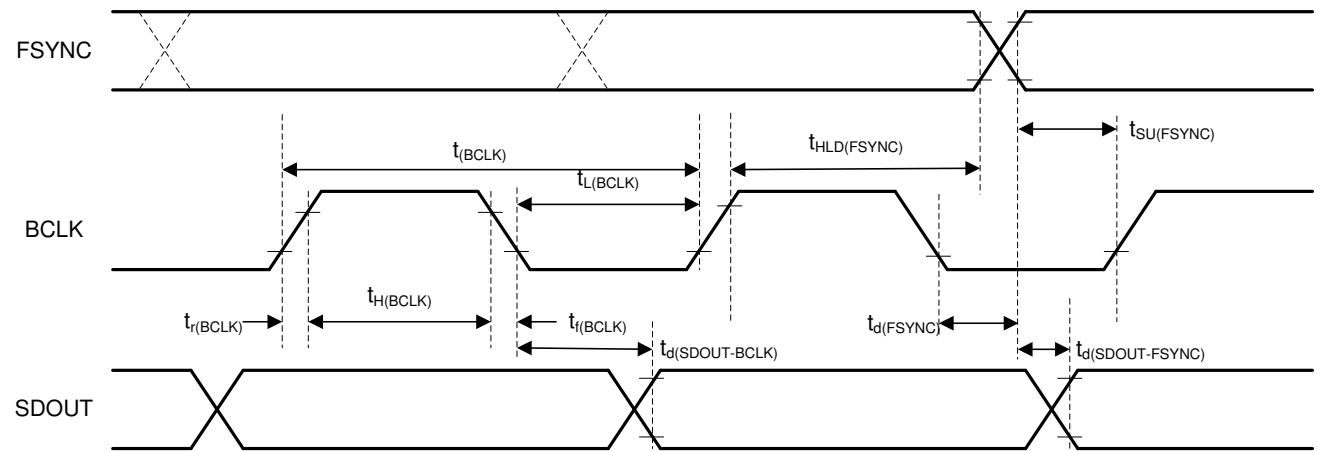
図 6-3. TDM (With BCLK_POL = 1), I²S, and LJ Interface Timing Diagram
