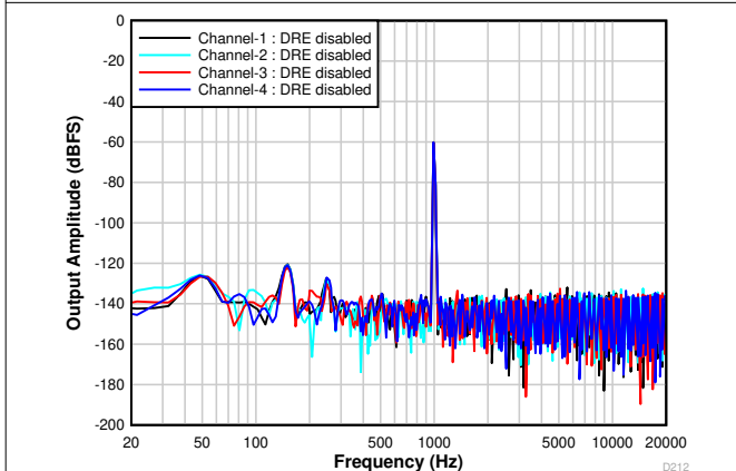
8-4. FFT With a -60-dBr Input With DRE Disabled
