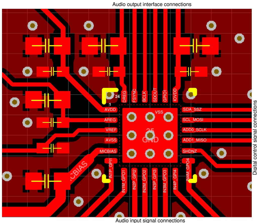
10-1. Layout Example
