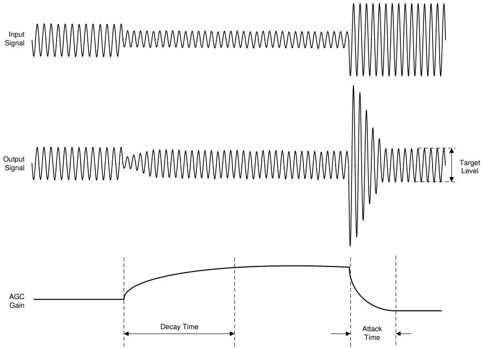
图 7-63. AGC Characteristics
