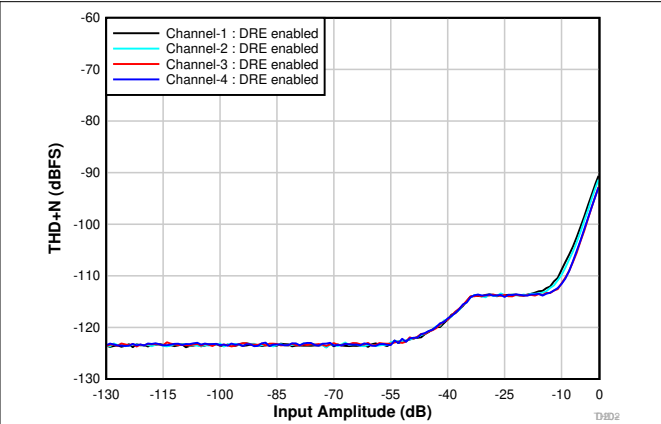
8-3. THD+N vs Input Amplitude With DRE Enabled
