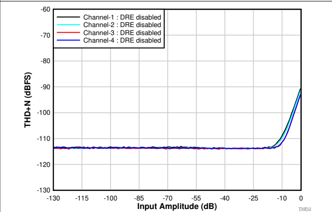
8-5. THD+N vs Input Amplitude With DRE Disabled
