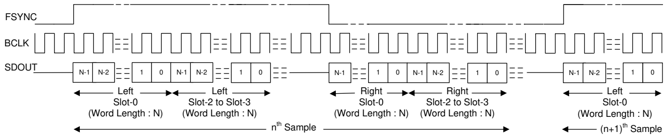
8-10. LJ Mode Standard Protocol Timing (TX_OFFSET = 0)
