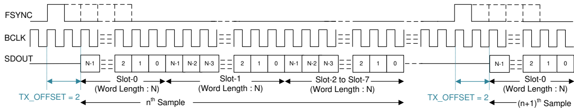
8-3. TDM Mode Protocol Timing (TX_OFFSET = 2)
