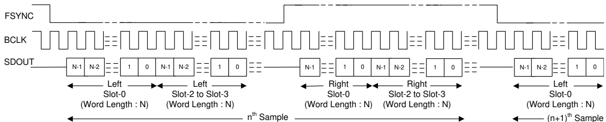
8-9. I 2 S Protocol Timing (TX_OFFSET = 0 and BCLK_POL = 1)
