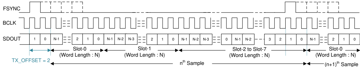
8-4. TDM Mode Protocol Timing (No Idle BCLK Cycles, TX_OFFSET = 2)
