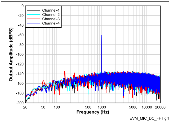
DC-coupled differential microphone input with DC common-mode 1N \times P = \sim 6\text{ V} and IN \times M = \sim 2\text{ V} , high swing mode enabled, measured using an external audio input source
