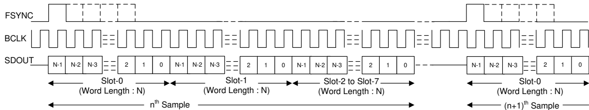
8-5. TDM Mode Protocol Timing (TX_OFFSET = 0 and BCLK_POL = 1)
