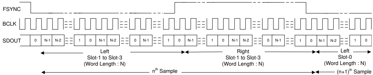
8-8. I 2 S Protocol Timing (No Idle BCLK Cycles, TX_OFFSET = 0)
