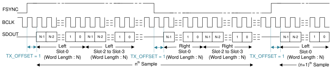
8-13. LJ Protocol Timing (TX_OFFSET = 1 and BCLK_POL = 1)
