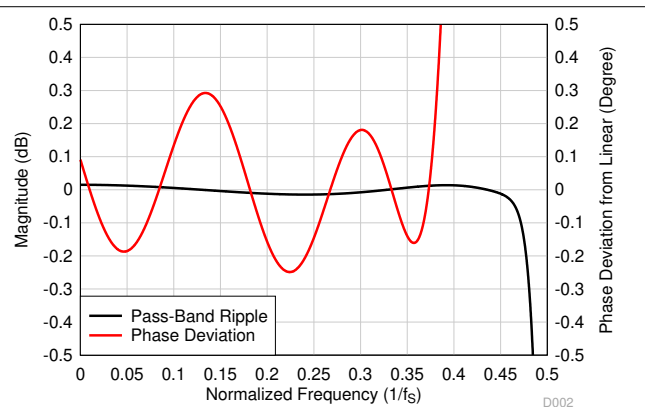
图 8-50. Low-Latency Decimation Filter Pass-Band Ripple and Phase Deviation
