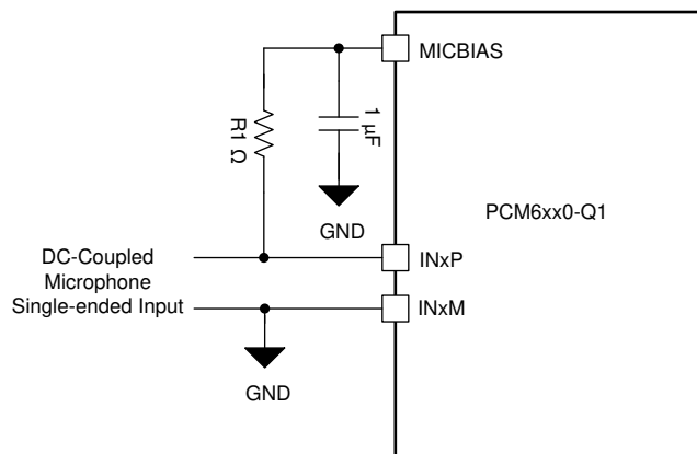
8-16. DC-Coupled Microphone Single-Ended Input Connection
