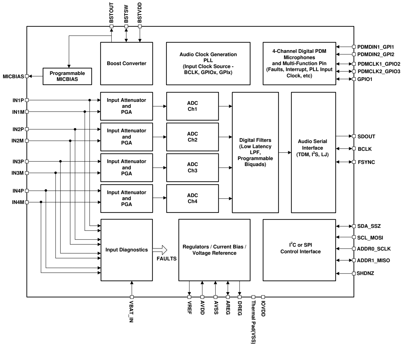
8-1. Simplified Device Functional Block Diagram
