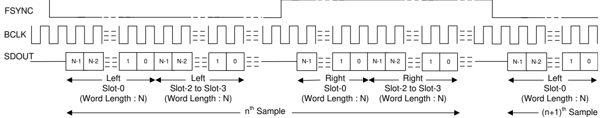
8-6. I 2 S Mode Standard Protocol Timing (TX_OFFSET = 0)
