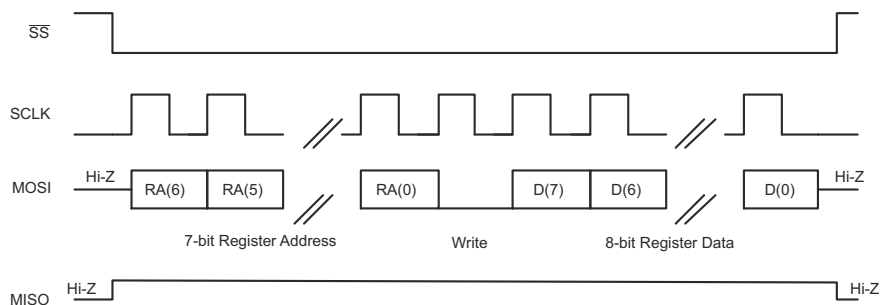
图 8-75. SPI Single-Byte Write Transfer
