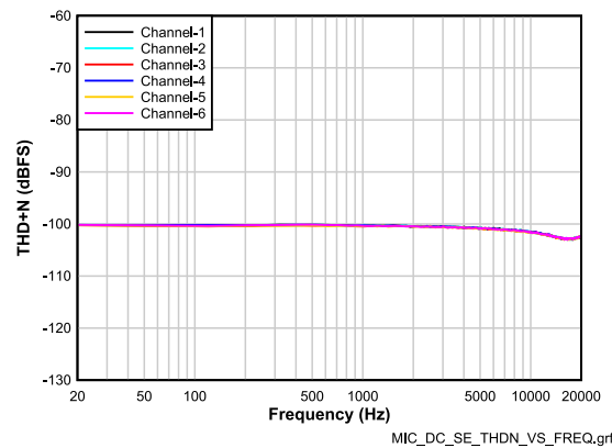
DC-coupled single-ended microphone input with DC common-mode 1N \times P = 4\text{ V} and IN \times M = 0\text{ V} , high swing mode enabled
