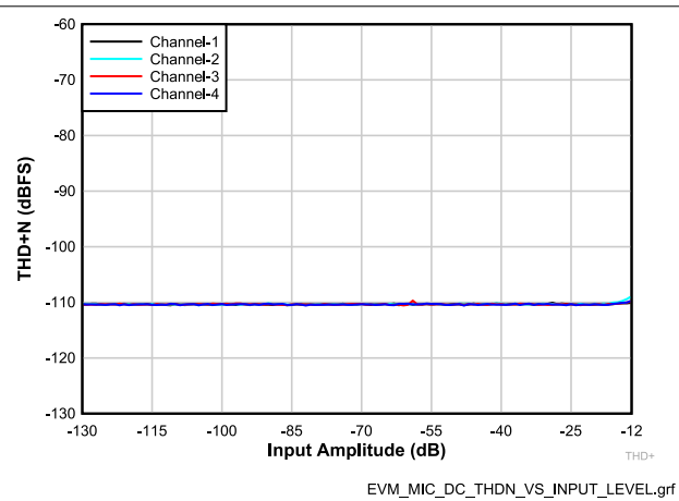
DC-coupled differential microphone input with DC common-mode 1N \times P = \sim 6\text{ V} and IN \times M = \sim 2\text{ V} , high swing mode enabled, measured using an external audio input source
