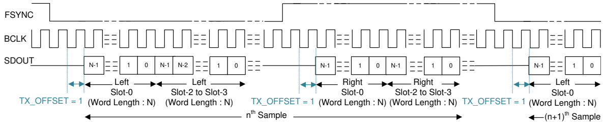
8-7. I 2 S Protocol Timing (TX_OFFSET = 1)
