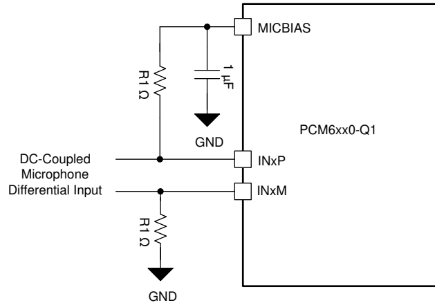
8-15. DC-Coupled Microphone Differential Input Connection
