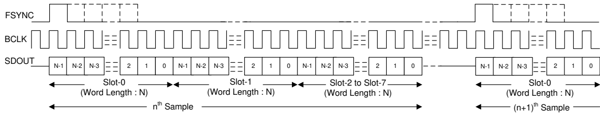
8-2. TDM Mode Standard Protocol Timing (TX_OFFSET = 0)
