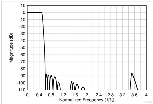
图 7-43. Low-Latency Decimation Filter Magnitude Response
