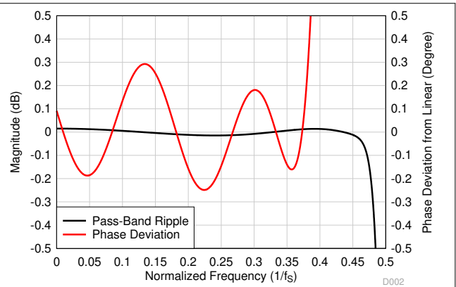
图 7-44. Low-Latency Decimation Filter Pass-Band Ripple and Phase Deviation
