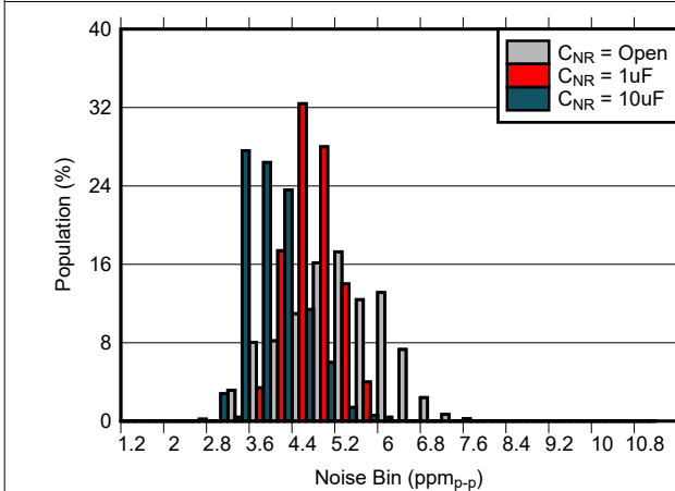
6-15. 0.1Hz to 10Hz Noise Distribution ( V_{REF} = 2.5\text{V} , C_L = 1\mu\text{F} , I_L = 0\text{mA} )
