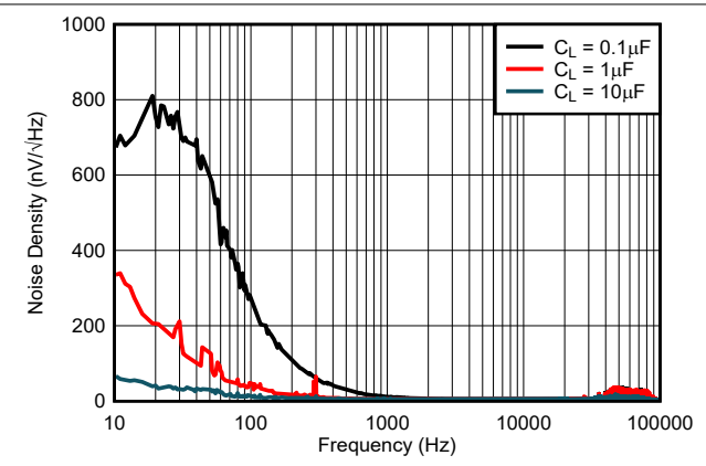
6-18. Noise Density vs Frequency ( V_{REF} = 2.5\text{V} , I_L = 0\text{mA} )
