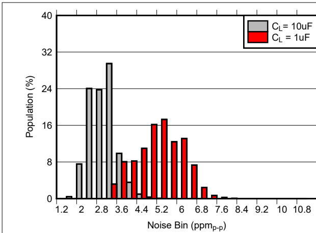
6-13. 0.1Hz to 10Hz Noise Distribution ( V_{REF} = 2.5\text{V} , C_{NR} = \text{Open} , I_L = 0\text{mA} )
