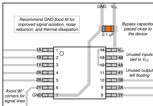
図 7-1. Layout Example for the SNx4AC00
