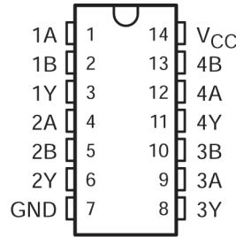
☒ 3-1. SN54AC00 J or W Package; SN74AC00 D, N, NS, or PW Package (Top View)
