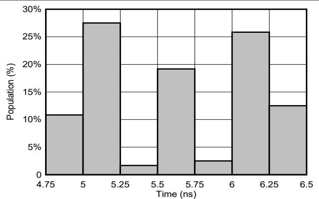
6-18. T PD Distribution; 5-V; T A = -55°C to 125°C (40 Samples)
