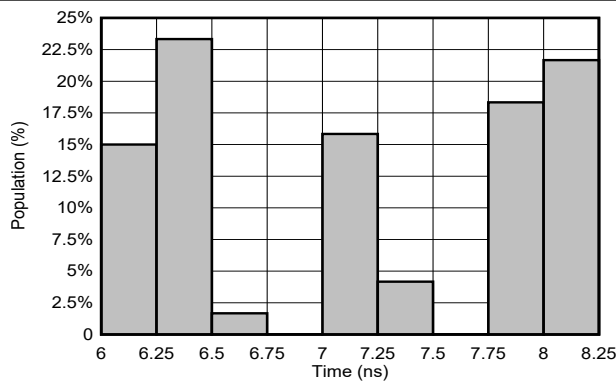
6-17. T PD Distribution; 3.3-V; T A = -55°C to 125°C (40 Samples)
