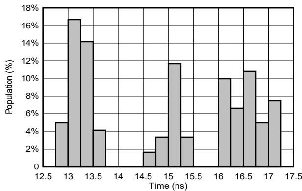
6-15. T PD Distribution; 1.8-V; T A = -55°C to 125°C (40 Samples)
