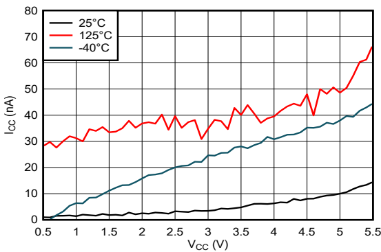
6-3. Supply Current Across Supply Voltage
