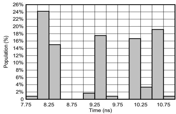
6-16. T PD Distribution; 2.5-V; T A = -55°C to 125°C (40 Samples)
