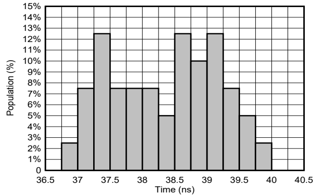
6-14. T PD Distribution; 1.2-V; T A = -55°C to 125°C (40 Samples)
