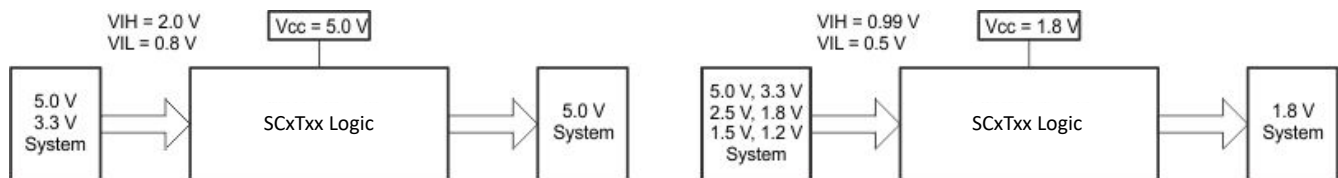
7-3. SCxT Up and Down Translation Example
