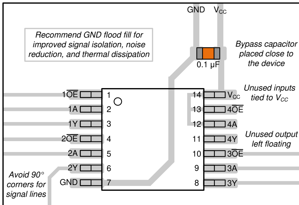
図 8-3. Example Layout for the SN74LV4T125-Q1
