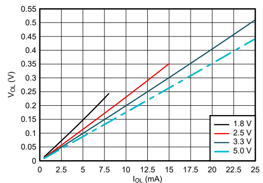
5-4. Output Voltage vs Current in LOW State
