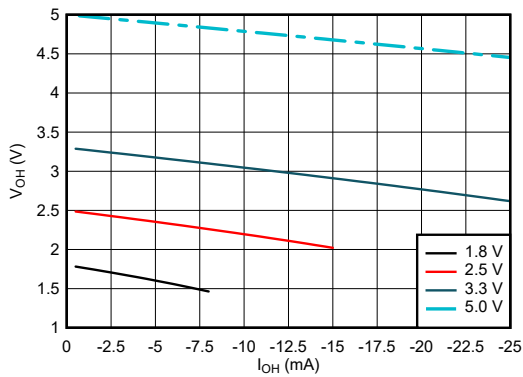
5-3. Output Voltage vs Current in HIGH State
