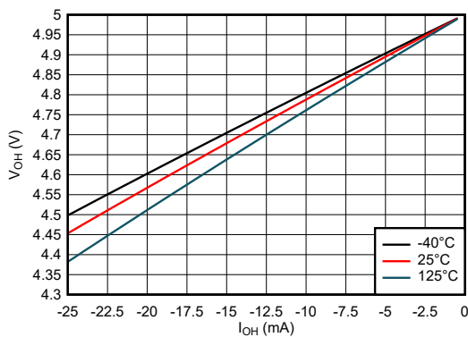
5-5. Output Voltage vs Current in HIGH State; 5-V Supply
