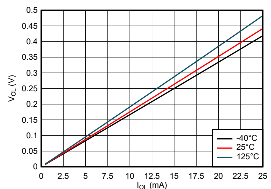
5-6. Output Voltage vs Current in LOW State; 5-V Supply
