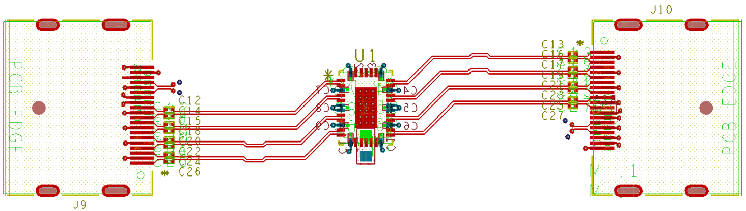
11-2. Example Layout (Top)
