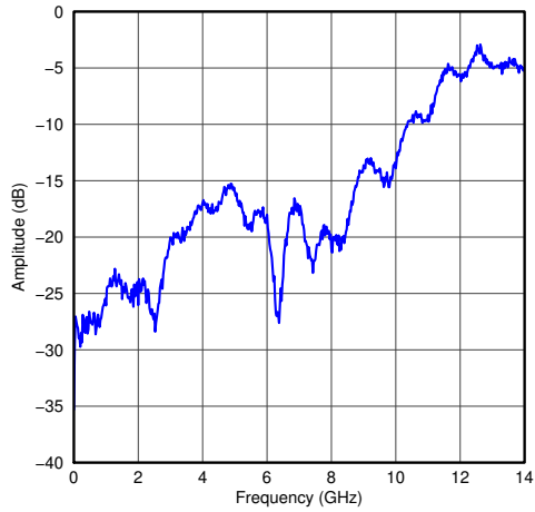
6-3. Differential Output Return Loss
