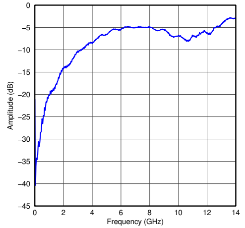
6-4. Common Mode Output Return Loss
