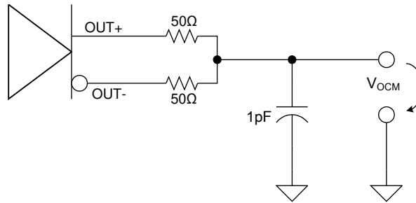
7-1. Common Mode Output Voltage Test Circuit
