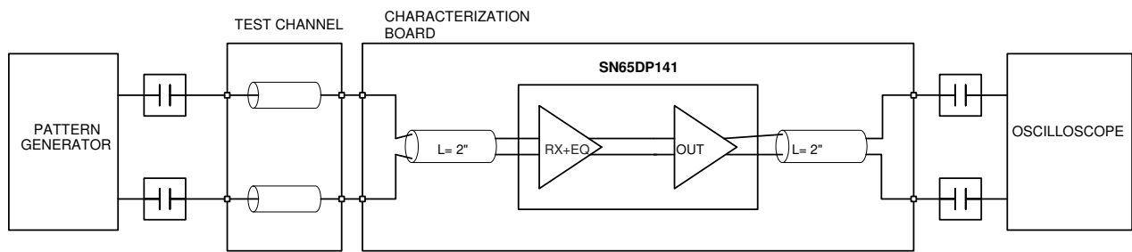
7-6. Receive Side Performance Test Circuit
