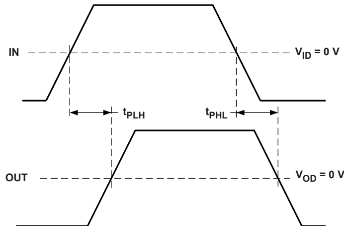
7-2. Propagation Delay Input to Output
