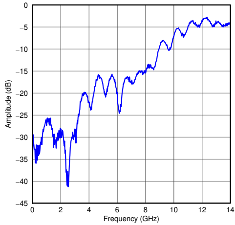
6-1. Differential Input Return Loss
