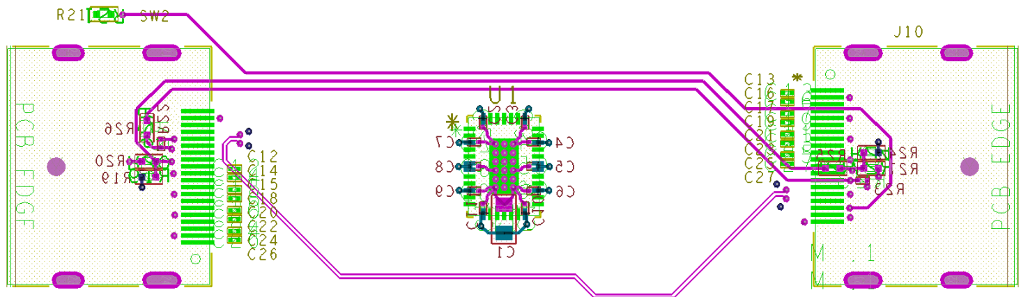
11-3. Example Layout (Top)
