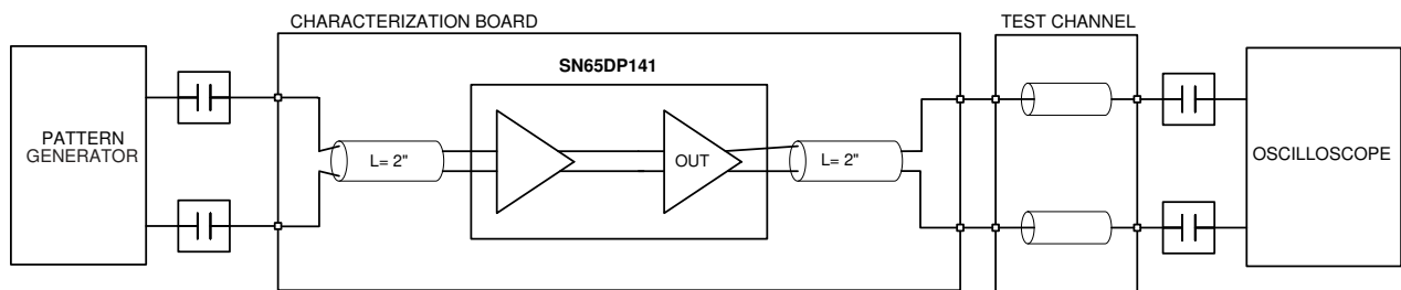
7-7. Transmit Side Performance Test Circuit
