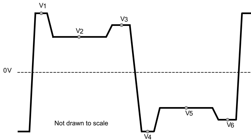
7-5. V_{(pre)} and V_{(post)} (test pattern is 1111111100000000 (8-1s, 8-0s))
