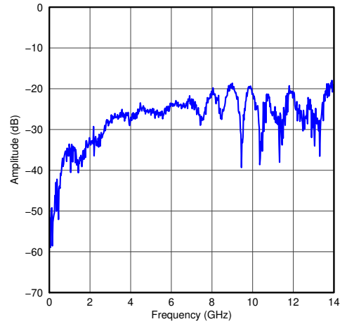
6-2. Differential to Common Mode Conversion
