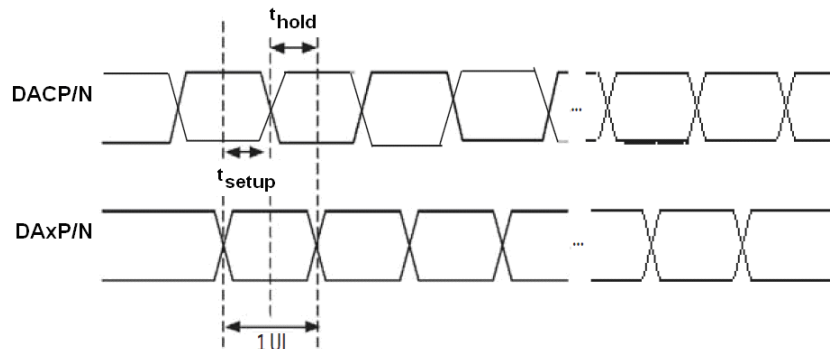
6-1. DSI HS Mode Receiver Timing Definitions
