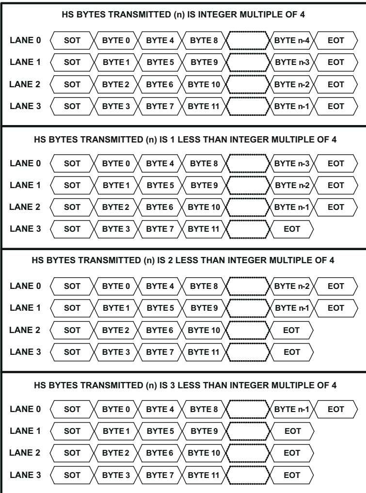
4 DSI Data Lane Configuration (default)
