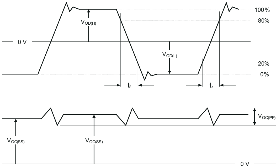
6-3. Test Load and Voltage Definitions for FlatLink Outputs
