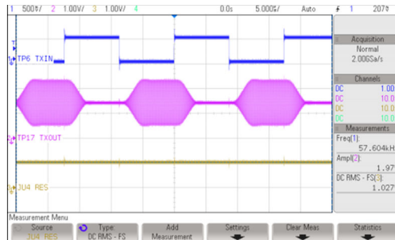
9-4. SN65HVD64 Application Curve
