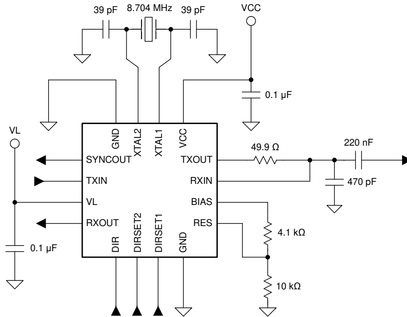
9-3. SN65HVD64 Schematic
