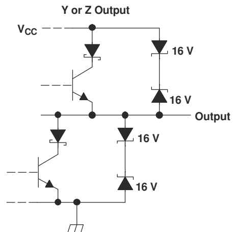
图 6-9. Equivalent Input and Output Schematic Diagrams
