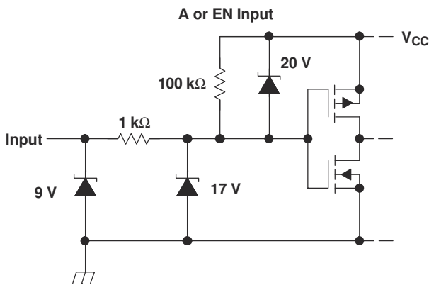
图 6-9. Equivalent Input and Output Schematic Diagrams
