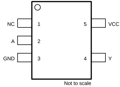
図 5-1. SN74AHC1G14-Q1 DBV Package, 5-Pin SOT-23; DCK Package, 5-Pin SC-70 (Top View)
