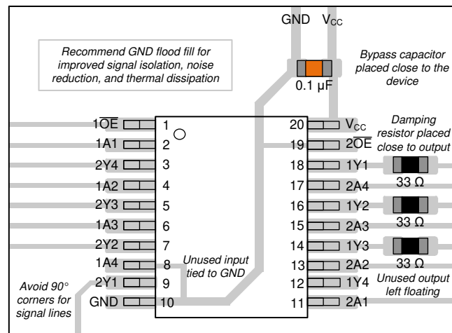
図 8-1. Example Layout for the SN74AHC244
