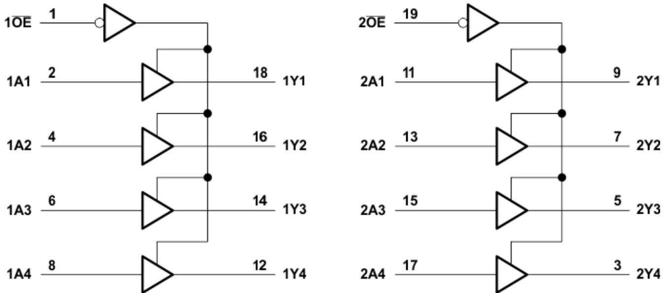
☒ 7-1. Logic Diagram (Positive Logic)
