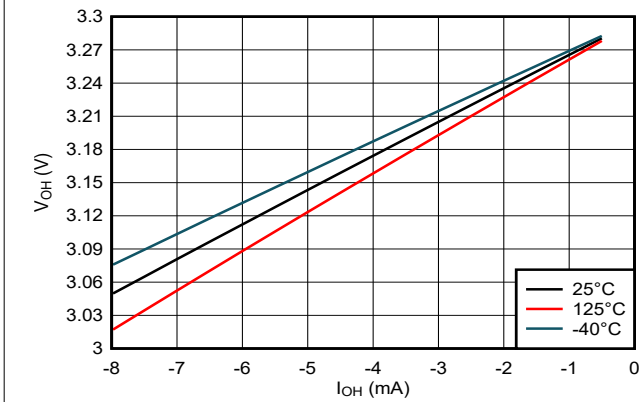
5-3. Output Voltage vs Current in HIGH State; 3.3-V Supply
