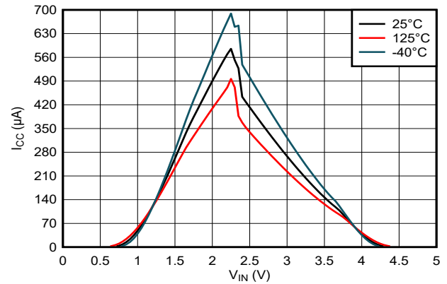
5-2. Supply Current Across Input Voltage; 5-V Supply
