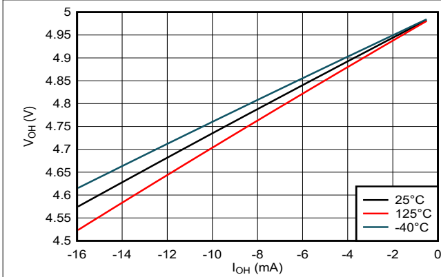
5-5. Output Voltage vs Current in HIGH State; 5-V Supply
