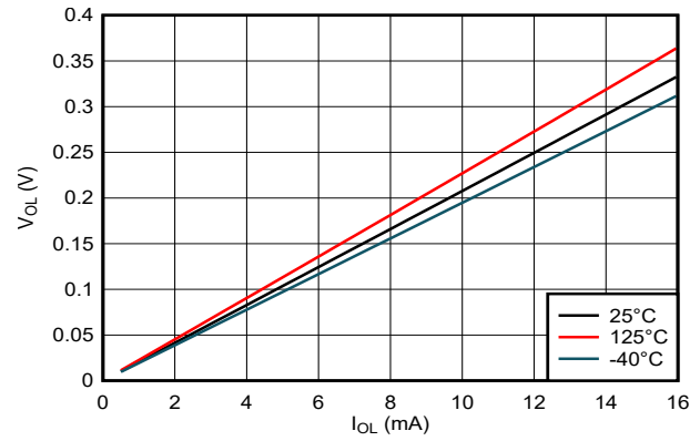
5-6. Output Voltage vs Current in LOW State; 5-V Supply
