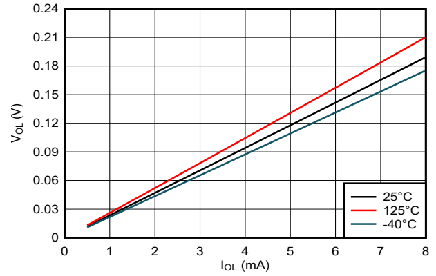
5-4. Output Voltage vs Current in LOW State; 3.3-V Supply
