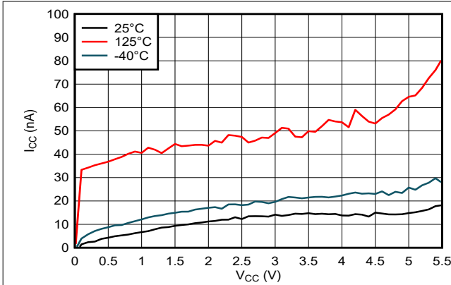
5-1. Supply Current Across Supply Voltage
