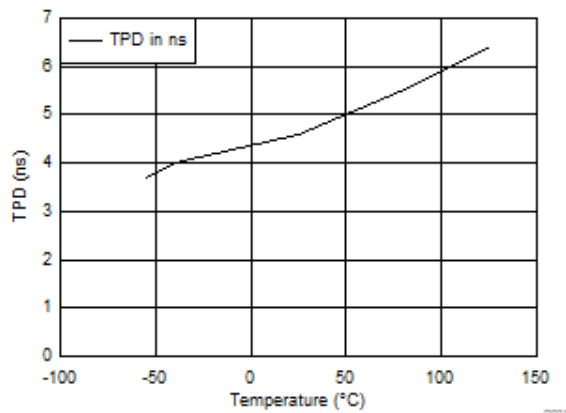
6-1. TPD vs Temperature, 15 pF Load
