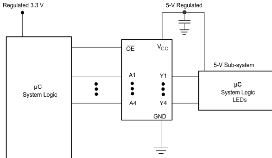
図 9-1. Specific Application Schematic
