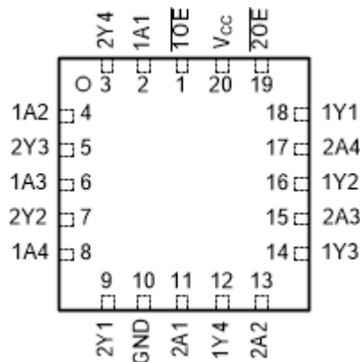
図 5-2. SN54AHCT244 FK Package (Top View)
