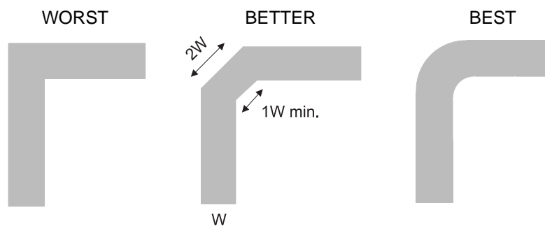
Figure 10. Trace Example
