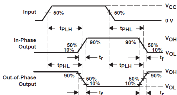
6-4. Voltage Waveforms Propagation Delay and Output Transition Times
