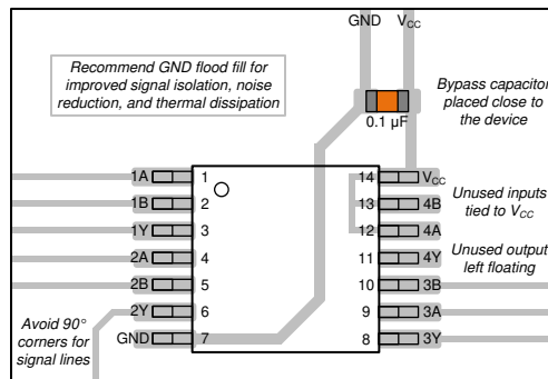
Figure 11 . Example layout for the SN74HCS7002-Q1
