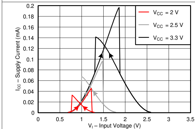
Fig 3. Typical supply current versus input voltage across common supply values (2 V to 3.3 V)
