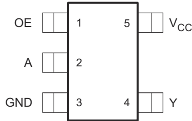
図 4-1. SN74LV1T126-Q1 DCK or DBV Package, 5-Pin SC70 or SOT-23 (Top View)
