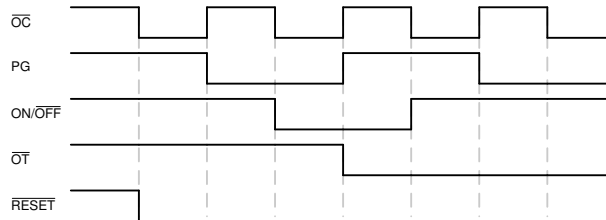
10-2. Application Timing Diagram
