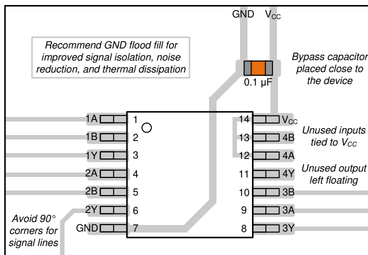
12-1. Example Layout for the SN74LV4T08-Q1
