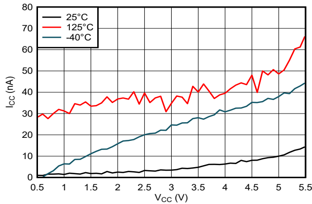
6-3. Supply Current Across Supply Voltage
