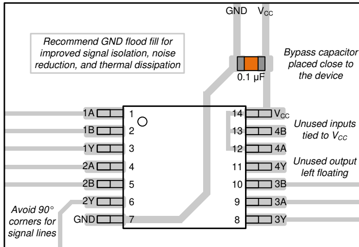
9-3. Example Layout for the SN74LV4T32
