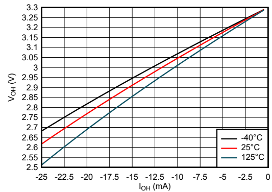
6-8. Output Voltage vs Current in HIGH State; 3.3-V Supply
