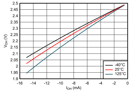
6-10. Output Voltage vs Current in HIGH State; 2.5-V Supply
