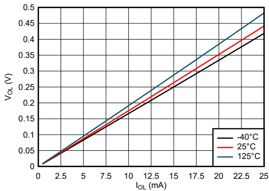
6-7. Output Voltage vs Current in LOW State; 5-V Supply
