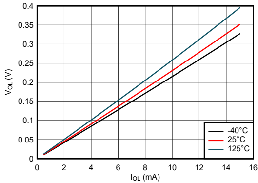
6-11. Output Voltage vs Current in LOW State; 2.5-V Supply
