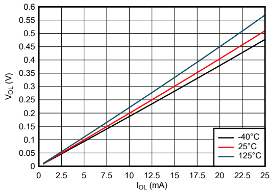
6-9. Output Voltage vs Current in LOW State; 3.3-V Supply
