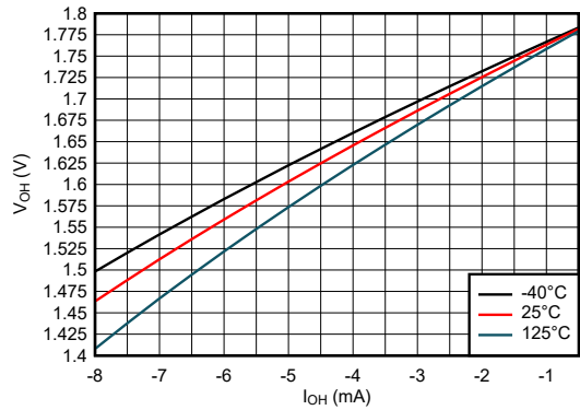
6-12. Output Voltage vs Current in HIGH State; 1.8-V Supply
