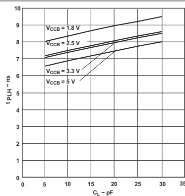
FIG 6-4. Typical Propagation Delay (B to A) vs Load Capacitance
