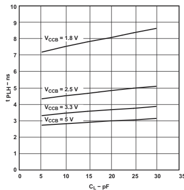
FIG 6-6. Typical Propagation Delay (A to B) vs Load Capacitance
