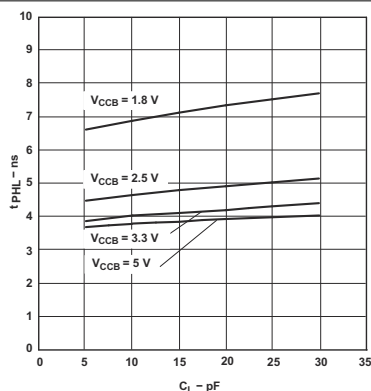
FIG 6-1. Typical Propagation Delay (A to B) vs Load Capacitance
