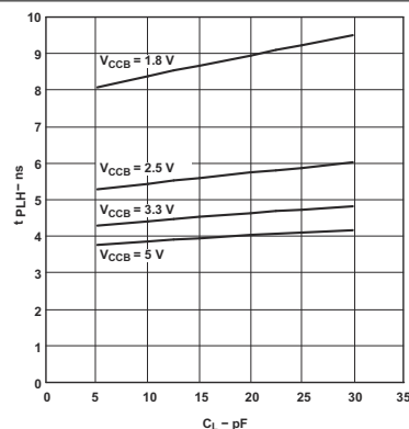
FIG 6-2. Typical Propagation Delay (A to B) vs Load Capacitance
