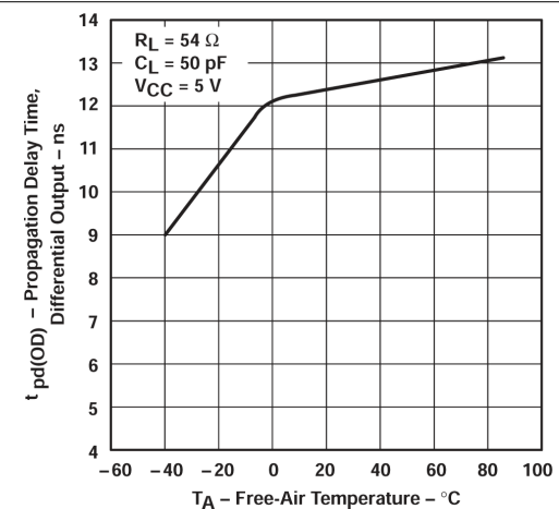
图 5-6. Propagation Delay Time, Differential Output vs Free-air Temperature
