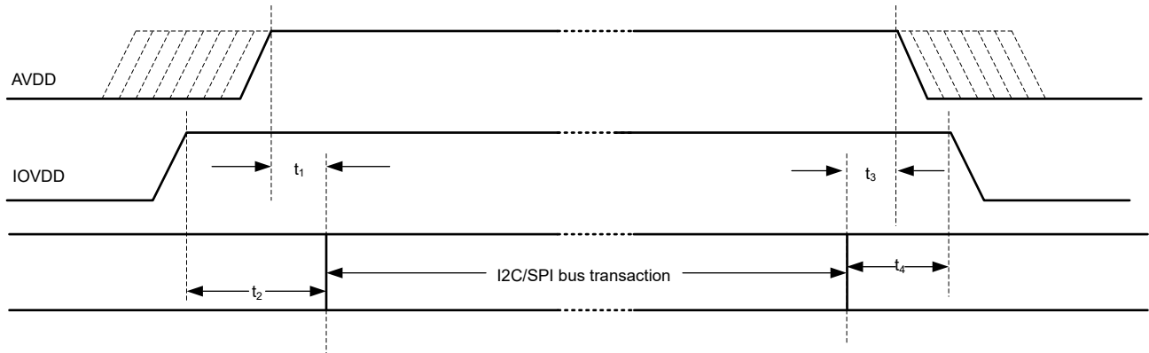
図 10-1. Power-Supply Sequencing Requirement Timing Diagram
