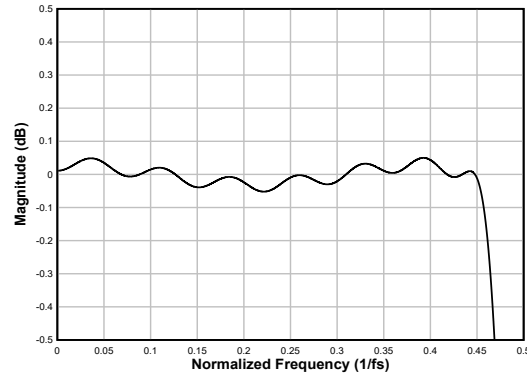
图 8-27. Linear Phase Decimation Filter Pass-Band Ripple
