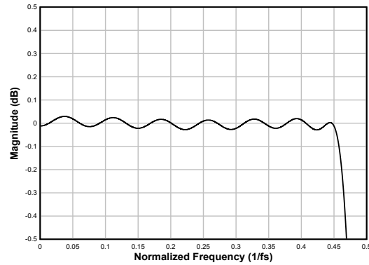
図 8-23. Linear Phase Interpolation Filter Pass-Band Ripple
