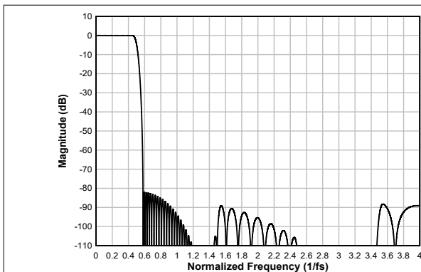
図 8-24. Linear Phase Interpolation Filter Magnitude Response
