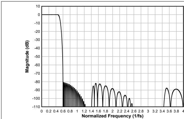
図 8-9. Linear Phase Decimation Filter Magnitude Response
