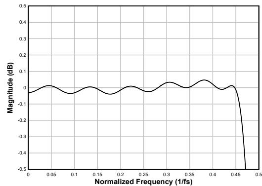
図 8-12. Linear Phase Decimation Filter Pass-Band Ripple
