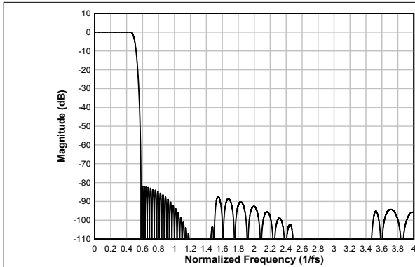
図 8-22. Linear Phase Interpolation Filter Magnitude Response
