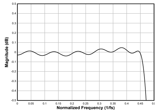
図 8-10. Linear Phase Decimation Filter Pass-Band Ripple
