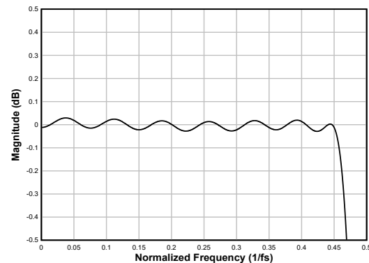
図 8-21. Linear Phase Interpolation Filter Pass-Band Ripple
