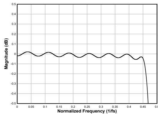
図 8-25. Linear Phase Interpolation Filter Pass-Band Ripple
