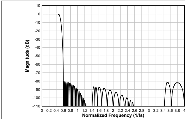
図 8-7. Linear Phase Decimation Filter Magnitude Response
