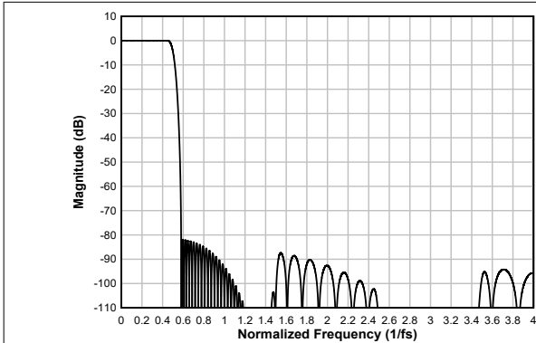
図 7-19. Linear Phase Interpolation Filter Magnitude Response
