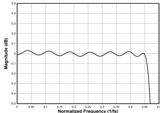
図 7-20. Linear Phase Interpolation Filter Pass-Band Ripple
