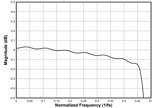
図 7-18. Linear Phase Interpolation Filter Pass-Band Ripple
