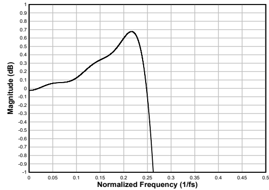
図 7-28. Linear Phase Interpolation Filter Pass-Band Ripple
