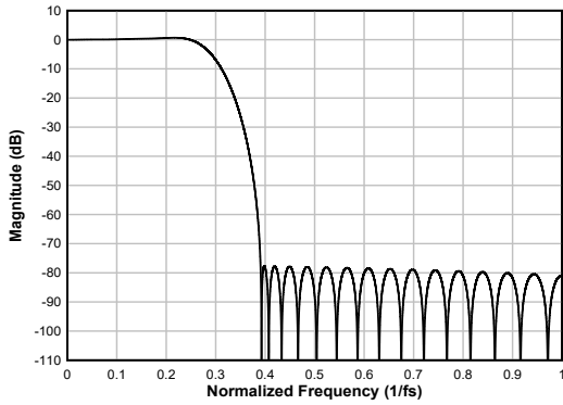
図 7-27. Linear Phase Interpolation Filter Magnitude Response
