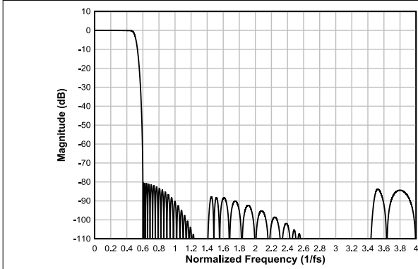
図 7-17. Linear Phase Interpolation Filter Magnitude Response
