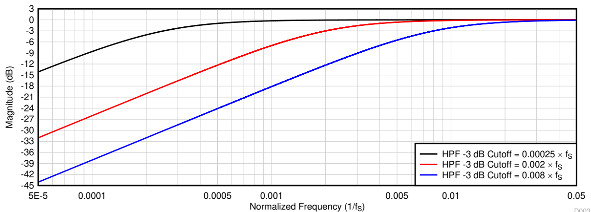
図 7-16. HPF Filter Frequency Response Plot
