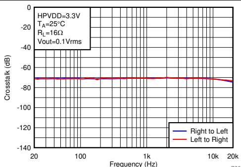
HPVDD = 3.3 V V_O = 0.1 Vrms Load = 16 \Omega
