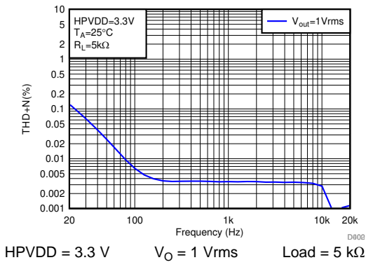
59. THD+N vs Frequency
