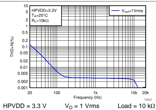
62. THD+N vs Frequency
