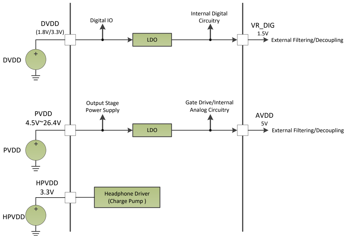
✕ 137. Power Supply Function Block Diagram
