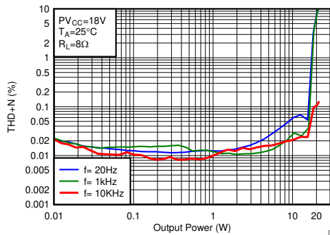
Figure 15. THD+N vs Output Power-BTL
