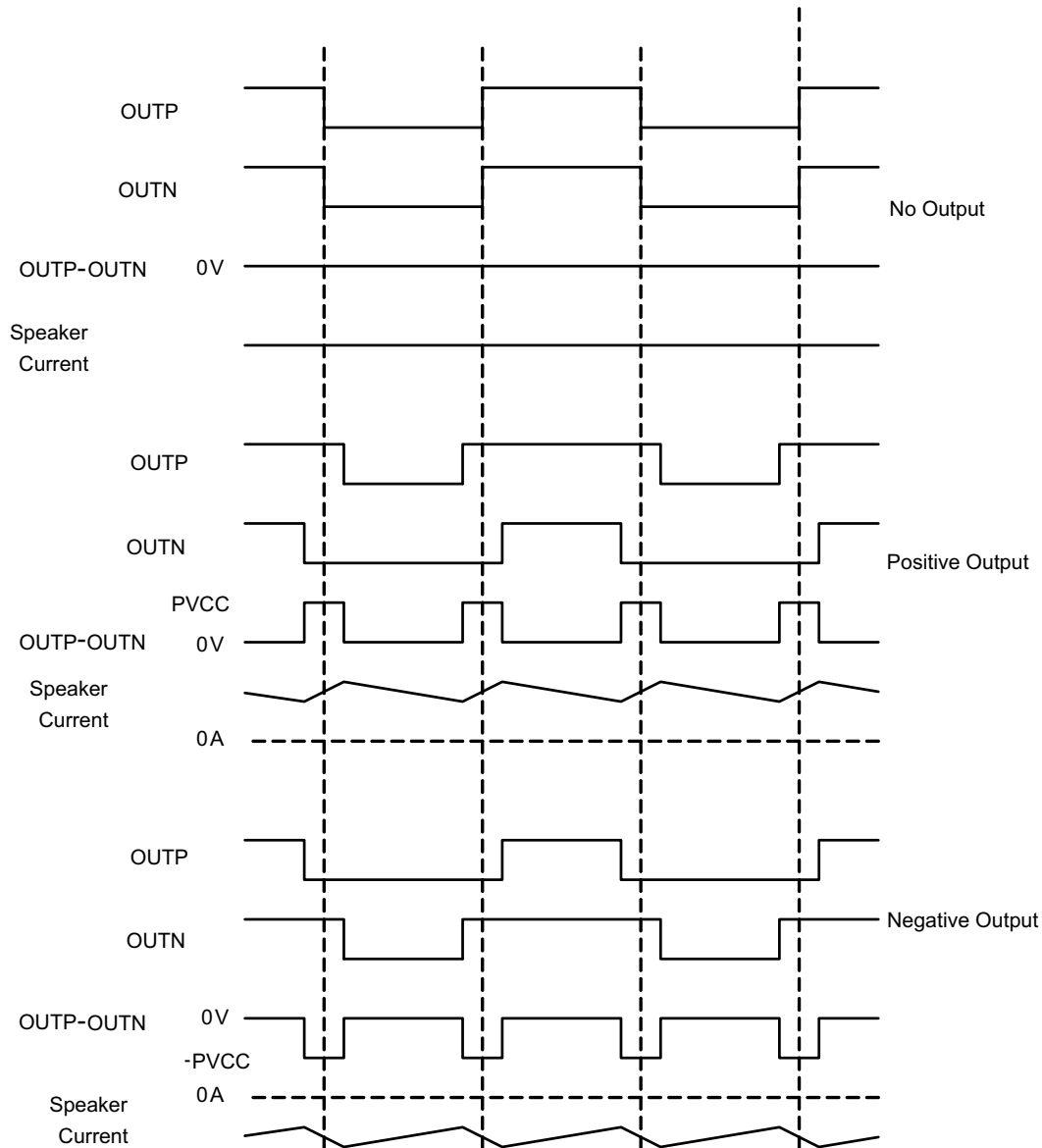
74. BD Mode Modulation
