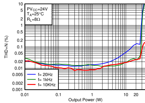
Figure 16. THD+N vs Output Power-BTL
