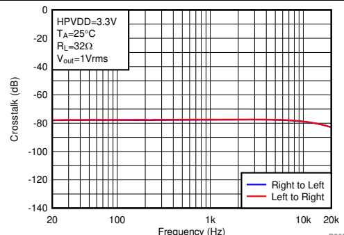
HPVDD = 3.3 V V_O = 1 Vrms Load = 32 \Omega
