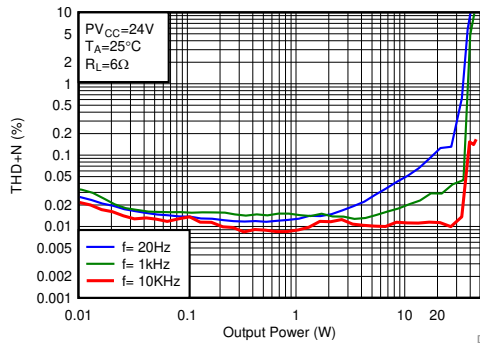
Figure 13. THD+N vs Output Power-BTL
