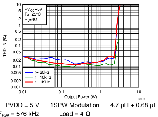
47. THD+N vs Output Power
