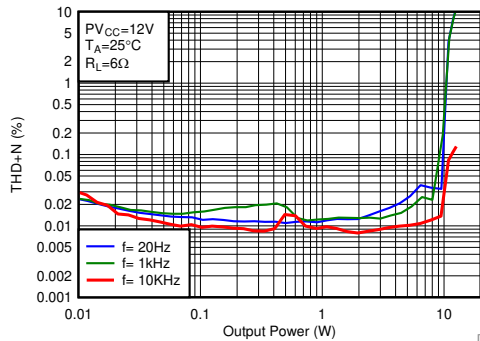
Figure 13. THD+N vs Output Power-BTL
