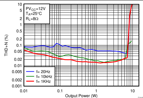
Fig 35. THD+N vs Output Power
