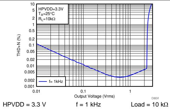
63. THD+N vs Output Voltage
