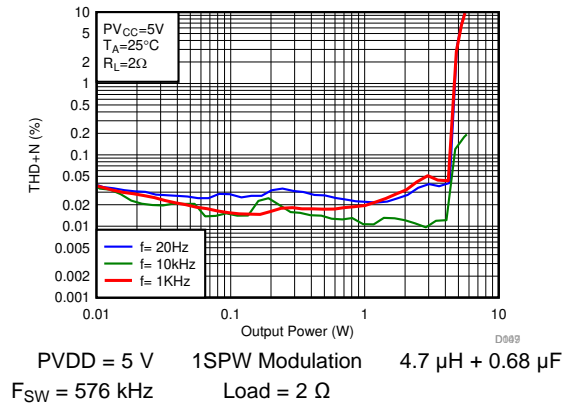
46. THD+N vs Output Power
