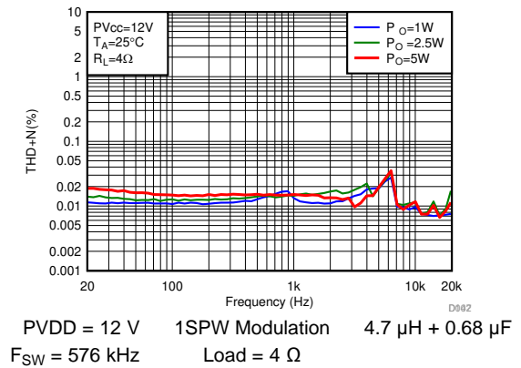
44. THD+N vs Frequency
