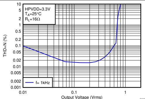
HPVDD = 3.3 V f = 1 kHz Load = 16 \Omega
