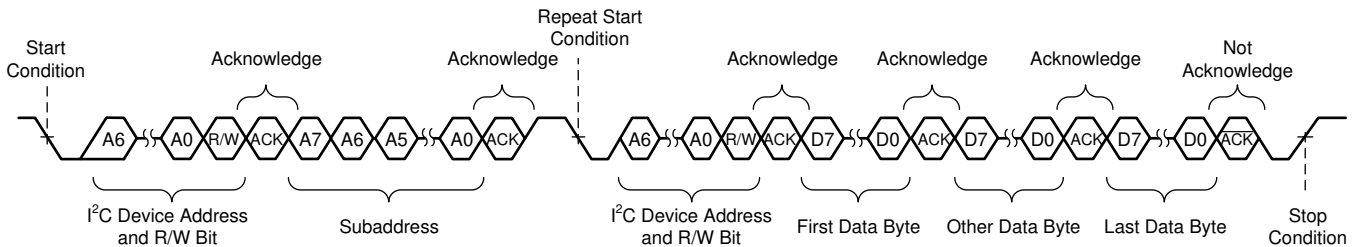
Figure 79. Sequential Read Transfer
