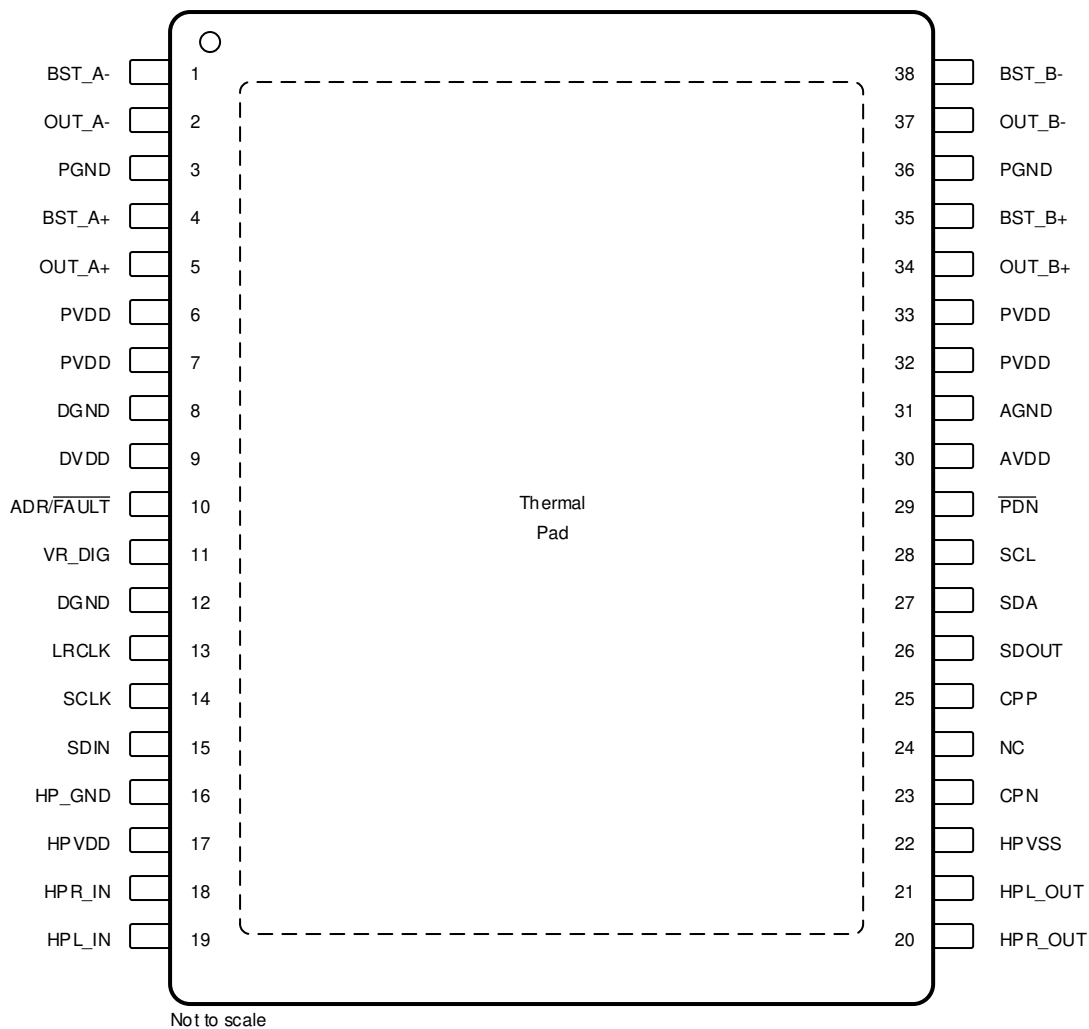
DCP Package 38-Pin TSSOP Top View
