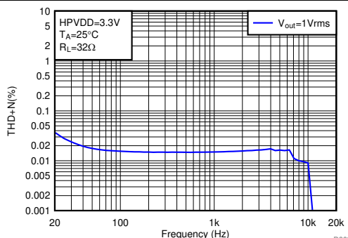
HPVDD = 3.3 V V_O = 1 Vrms Load = 32 \Omega
