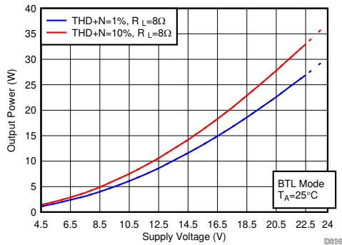
19. Output Power vs Supply Voltage
