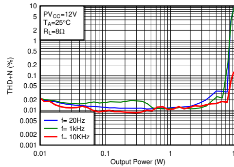
Figure 14. THD+N vs Output Power-BTL
