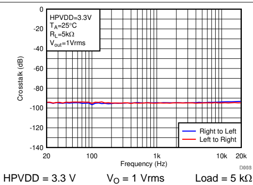
61. Crosstalk vs Frequency
