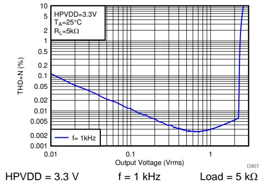
60. THD+N vs Output Voltage
