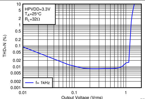
HPVDD = 3.3 V f = 1 kHz Load = 32 \Omega
