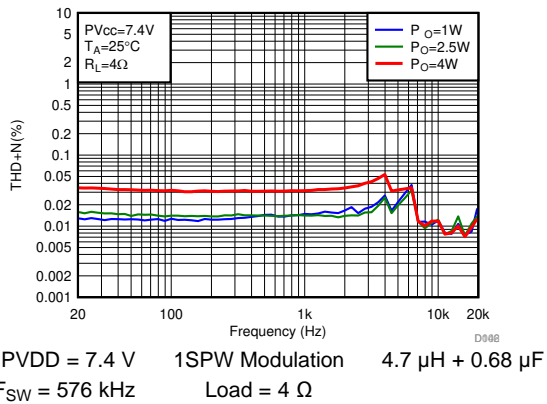
43. THD+N vs Frequency
