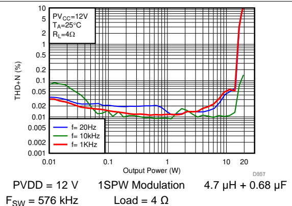
48. THD+N vs Output Power
