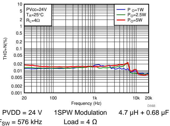
45. THD+N vs Frequency
