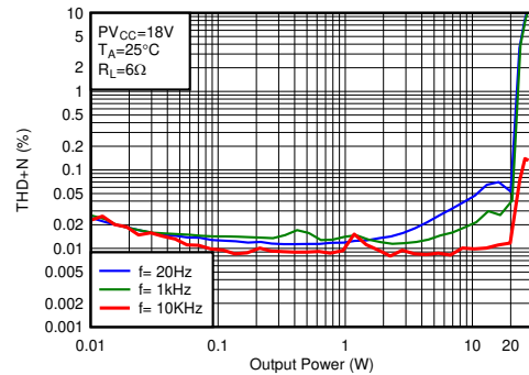
Figure 14. THD+N vs Output Power-BTL
